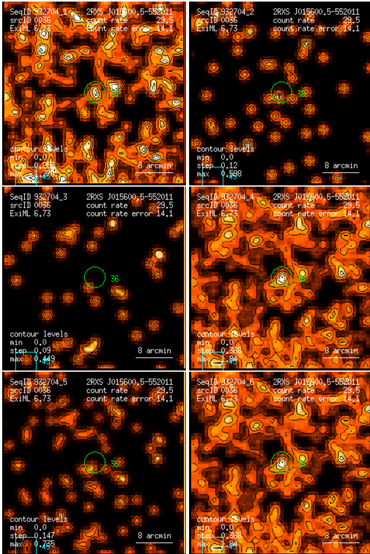
Figure 36: RASS 932704: detection 0036: band rate images, Gaussian filter: (1) PSPC channels 11 – 41, (2) 52 – 90, (3) 91 – 201, (4) 11 – 235, (5) 52 – 201, (6) 11 – 201. Broad band rates in counts/ks. Band rate contour levels in counts/ks/arcmin 2 .
