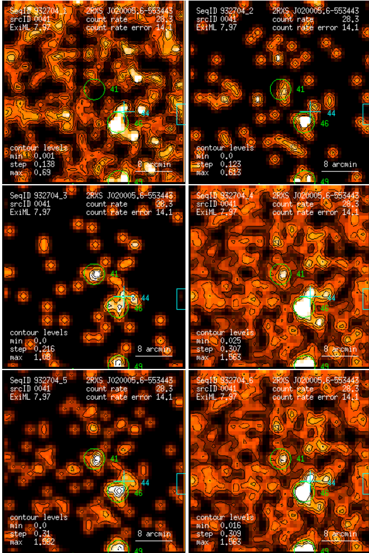
Figure 41: RASS 932704: detection 0041: band rate images, Gaussian filter: (1) PSPC channels 11 – 41, (2) 52 – 90, (3) 91 – 201, (4) 11 – 235, (5) 52 – 201, (6) 11 – 201. Broad band rates in counts/ks. Band rate contour levels in counts/ks/arcmin 2 .
