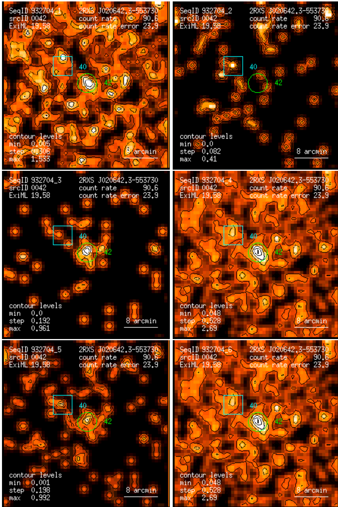
Figure 42: RASS 932704: detection 0042: band rate images, Gaussian filter: (1) PSPC channels 11 – 41, (2) 52 – 90, (3) 91 – 201, (4) 11 – 235, (5) 52 – 201, (6) 11 – 201. Broad band rates in counts/ks. Band rate contour levels in counts/ks/arcmin 2 .
