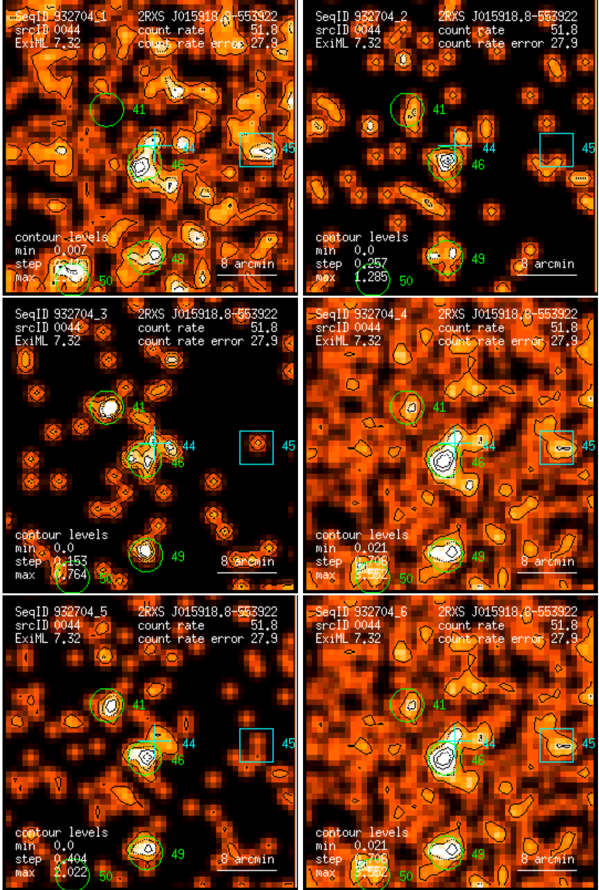
Figure 44: RASS 932704: detection 0044: band rate images, Gaussian filter: (1) PSPC channels 11 – 41, (2) 52 – 90, (3) 91 – 201, (4) 11 – 235, (5) 52 – 201, (6) 11 – 201. Broad band rates in counts/ks. Band rate contour levels in counts/ks/arcmin 2 .
