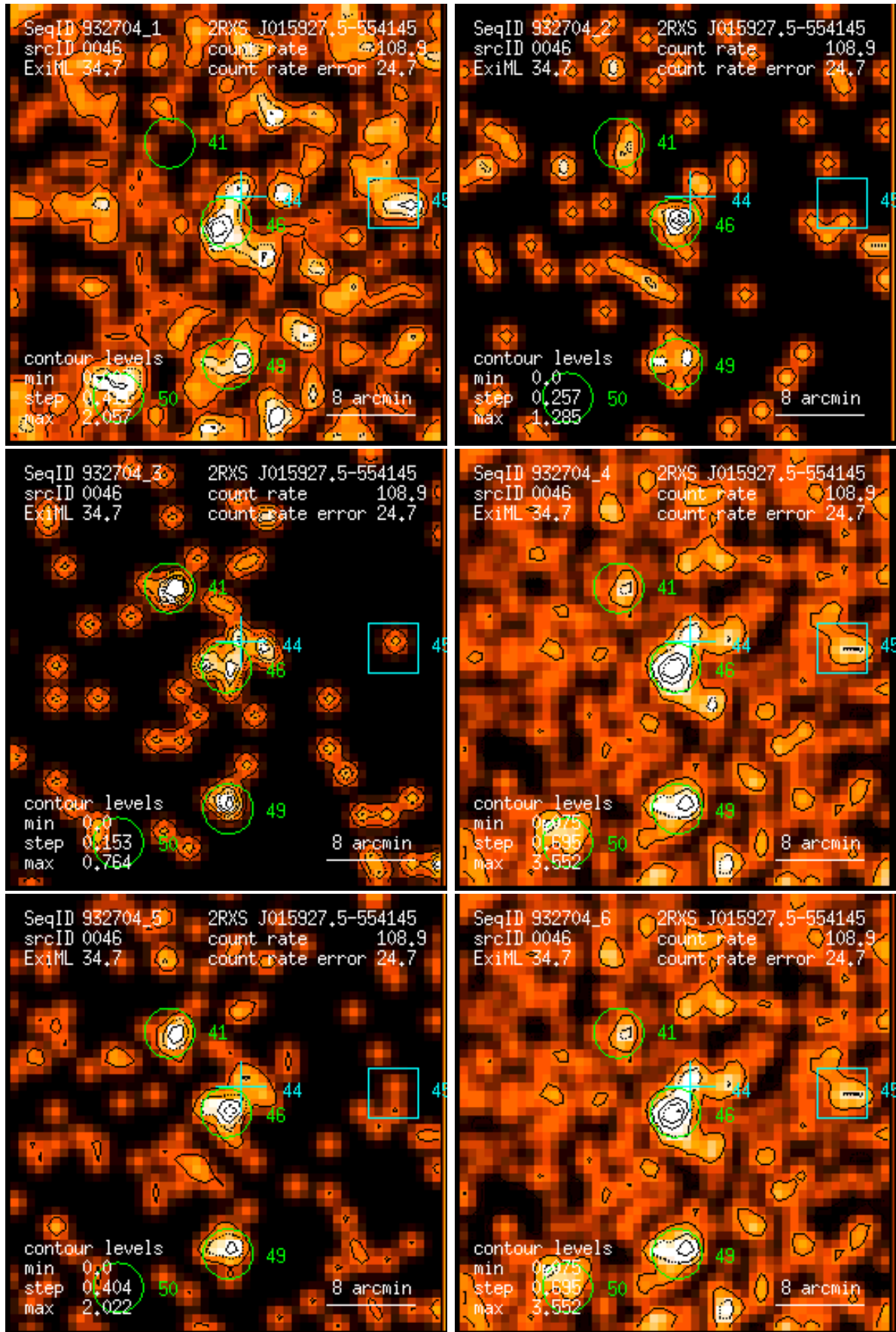
Figure 46: RASS 932704: detection 0046: band rate images, Gaussian filter: (1) PSPC channels 11 – 41, (2) 52 – 90, (3) 91 – 201, (4) 11 – 235, (5) 52 – 201, (6) 11 – 201. Broad band rates in counts/ks. Band rate contour levels in counts/ks/arcmin 2 .
