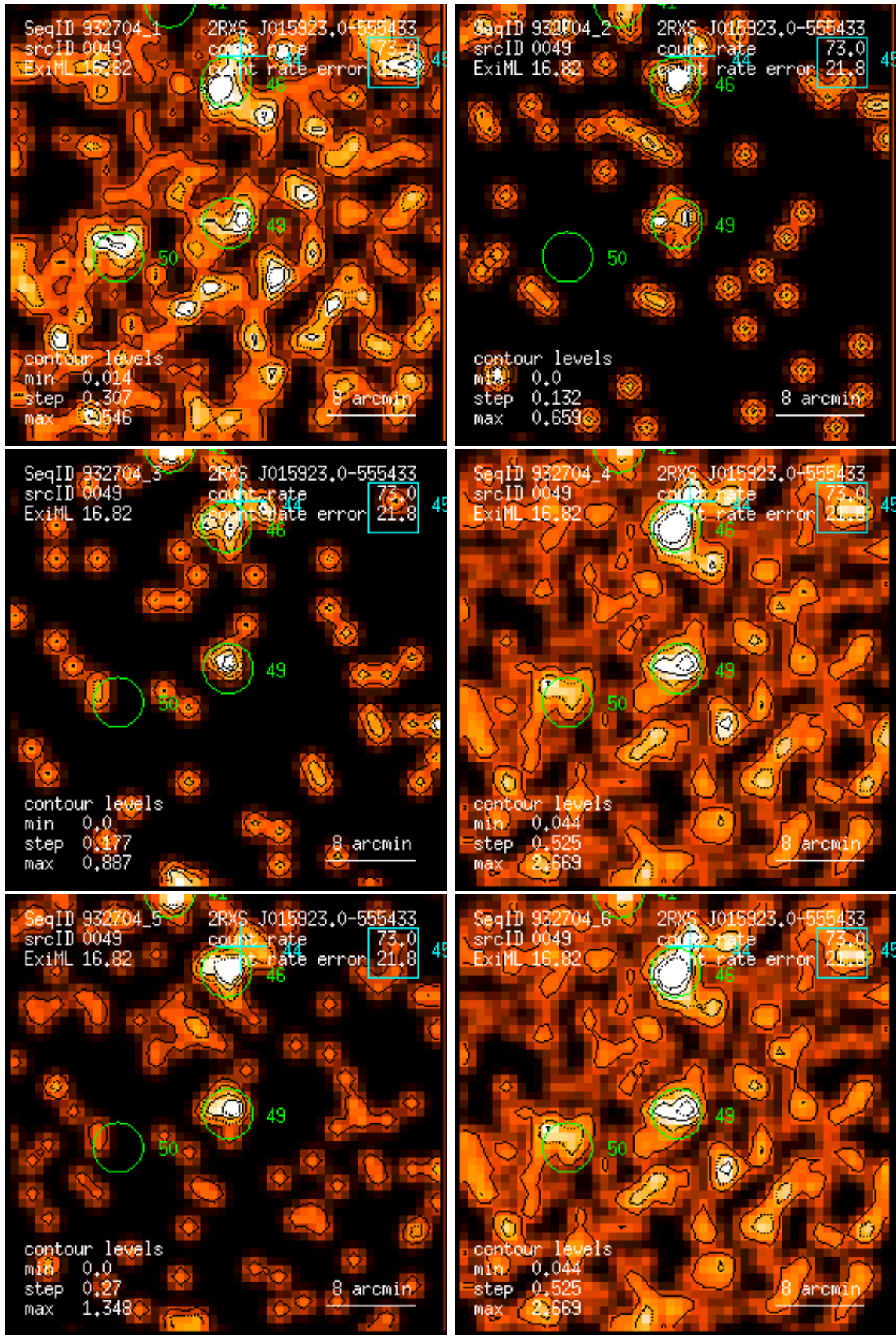
Figure 49: RASS 932704: detection 0049: band rate images, Gaussian filter: (1) PSPC channels 11 – 41, (2) 52 – 90, (3) 91 – 201, (4) 11 – 235, (5) 52 – 201, (6) 11 – 201. Broad band rates in counts/ks. Band rate contour levels in counts/ks/arcmin 2 .
