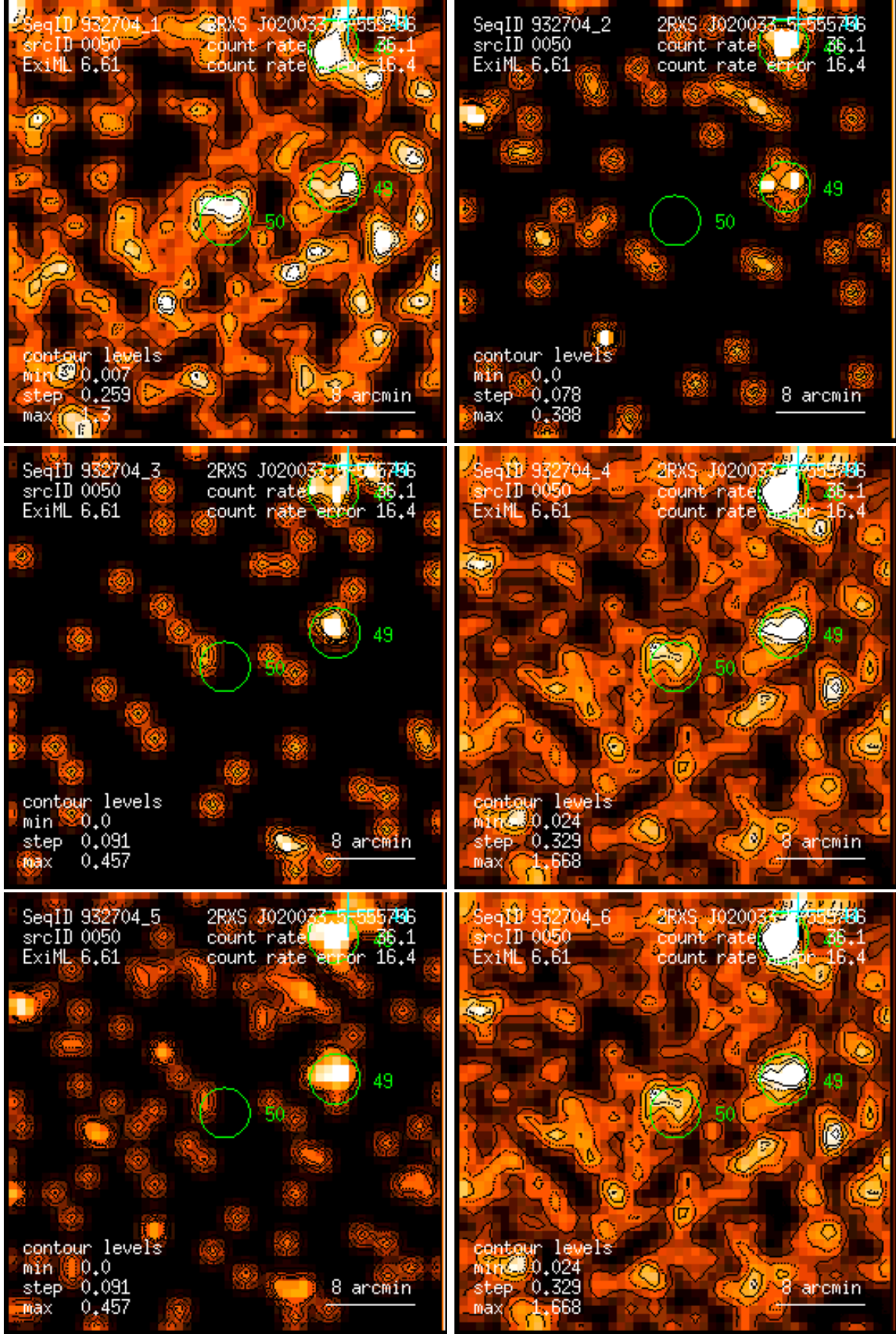
Figure 50: RASS 932704: detection 0050: band rate images, Gaussian filter: (1) PSPC channels 11 – 41, (2) 52 – 90, (3) 91 – 201, (4) 11 – 235, (5) 52 – 201, (6) 11 – 201. Broad band rates in counts/ks. Band rate contour levels in counts/ks/arcmin 2 .
