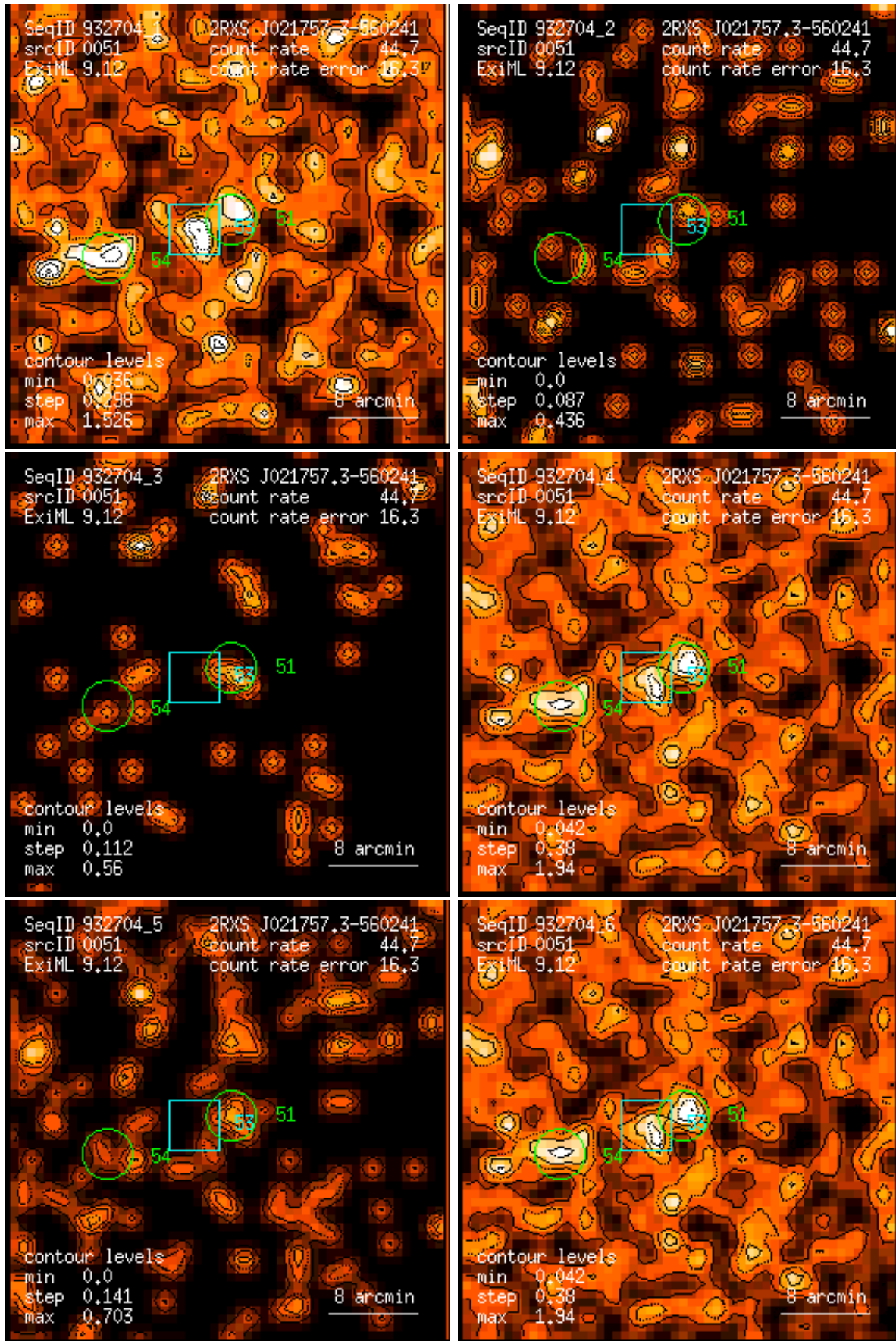
Figure 51: RASS 932704: detection 0051: band rate images, Gaussian filter: (1) PSPC channels 11 – 41, (2) 52 – 90, (3) 91 – 201, (4) 11 – 235, (5) 52 – 201, (6) 11 – 201. Broad band rates in counts/ks. Band rate contour levels in counts/ks/arcmin 2 .
