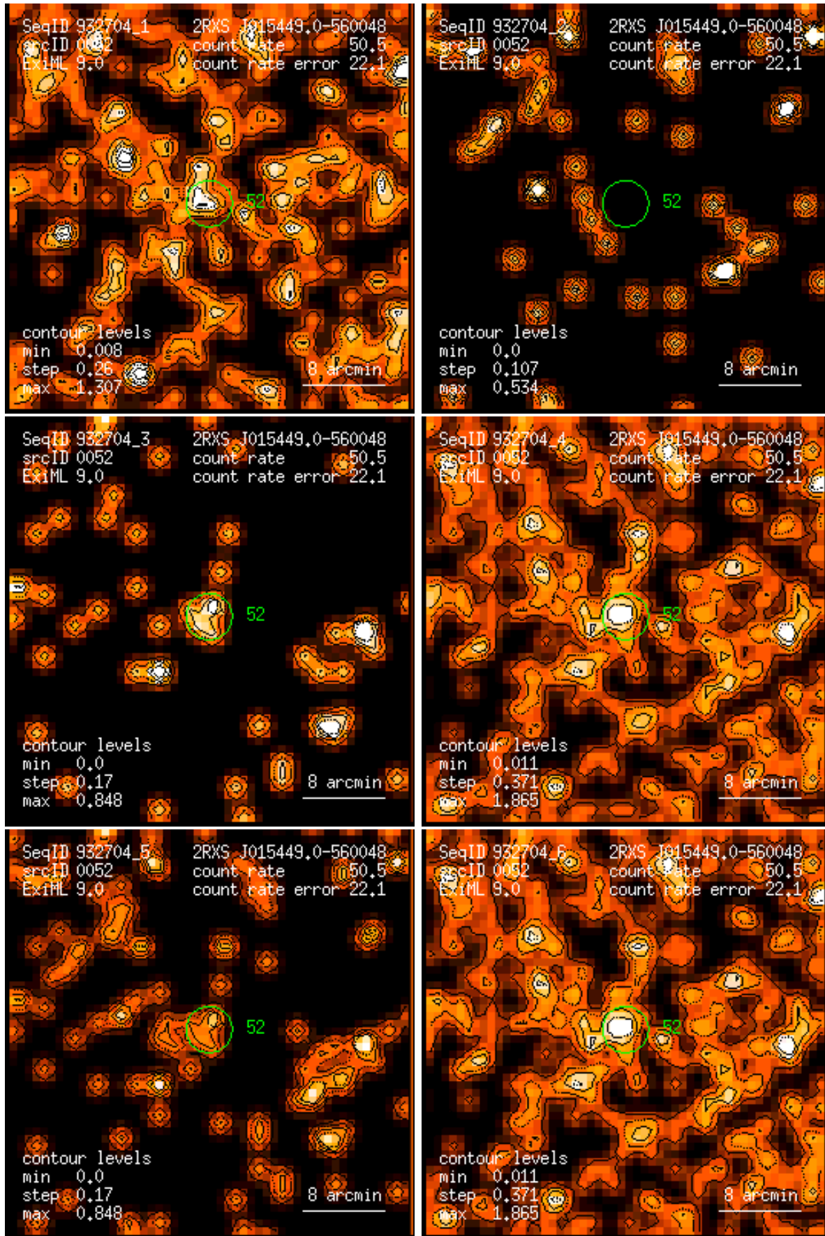
Figure 52: RASS 932704: detection 0052: band rate images, Gaussian filter: (1) PSPC channels 11 – 41, (2) 52 – 90, (3) 91 – 201, (4) 11 – 235, (5) 52 – 201, (6) 11 – 201. Broad band rates in counts/ks. Band rate contour levels in counts/ks/arcmin 2 .
