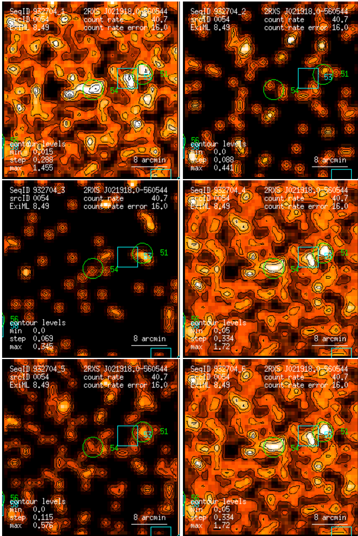
Figure 54: RASS 932704: detection 0054: band rate images, Gaussian filter: (1) PSPC channels 11 – 41, (2) 52 – 90, (3) 91 – 201, (4) 11 – 235, (5) 52 – 201, (6) 11 – 201. Broad band rates in counts/ks. Band rate contour levels in counts/ks/arcmin 2 .
