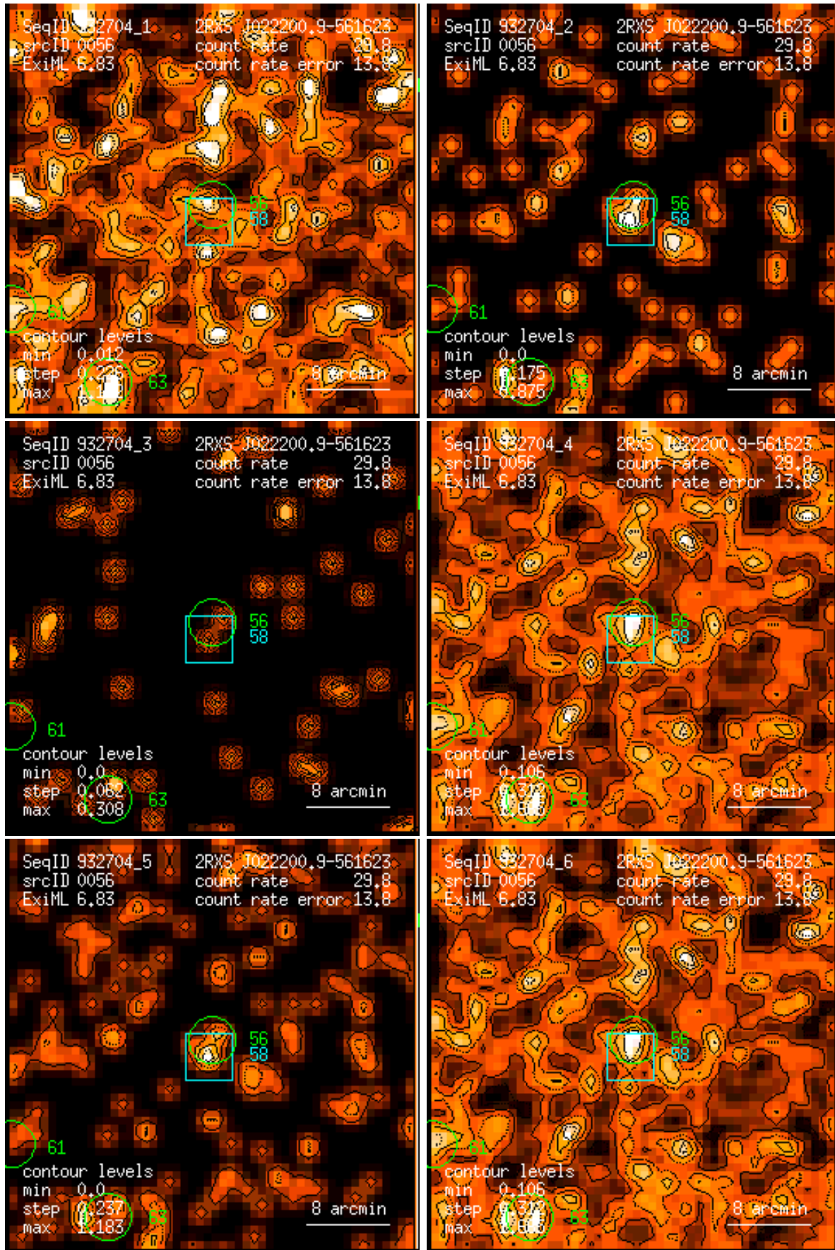
Figure 56: RASS 932704: detection 0056: band rate images, Gaussian filter: (1) PSPC channels 11 – 41, (2) 52 – 90, (3) 91 – 201, (4) 11 – 235, (5) 52 – 201, (6) 11 – 201. Broad band rates in counts/ks. Band rate contour levels in counts/ks/arcmin 2 .
