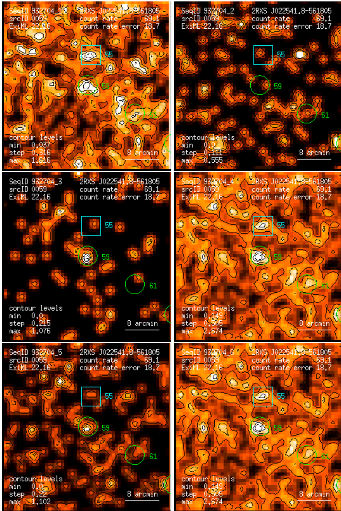
Figure 59: RASS 932704: detection 0059: band rate images, Gaussian filter: (1) PSPC channels 11 – 41, (2) 52 – 90, (3) 91 – 201, (4) 11 – 235, (5) 52 – 201, (6) 11 – 201. Broad band rates in counts/ks. Band rate contour levels in counts/ks/arcmin 2 .
