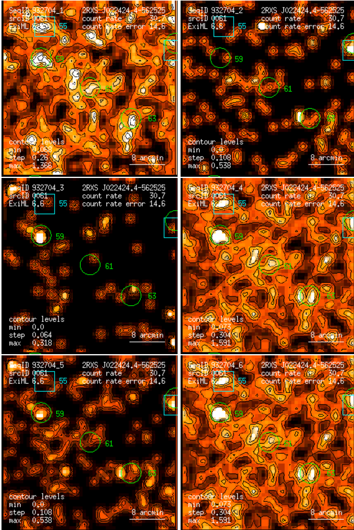
Figure 61: RASS 932704: detection 0061: band rate images, Gaussian filter: (1) PSPC channels 11 – 41, (2) 52 – 90, (3) 91 – 201, (4) 11 – 235, (5) 52 – 201, (6) 11 – 201. Broad band rates in counts/ks. Band rate contour levels in counts/ks/arcmin 2 .
