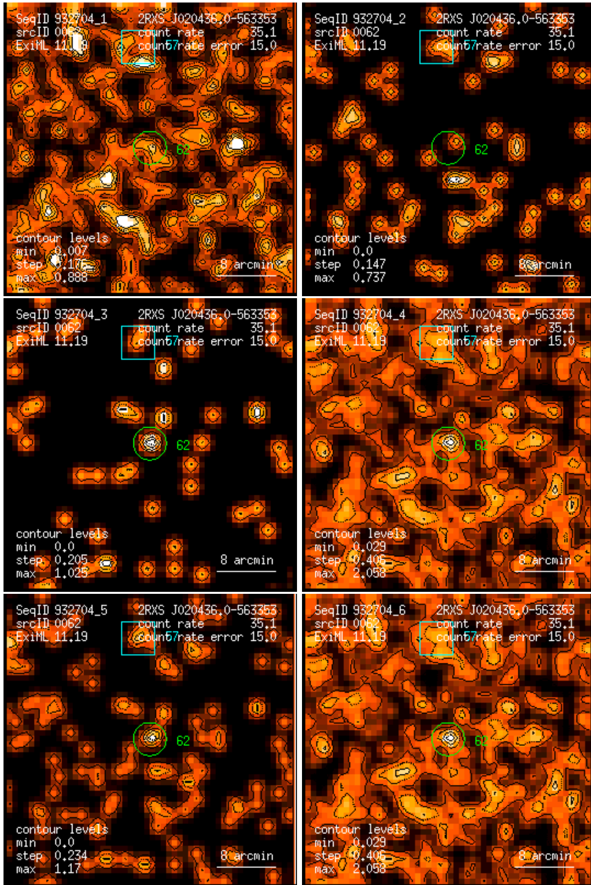
Figure 62: RASS 932704: detection 0062: band rate images, Gaussian filter: (1) PSPC channels 11 – 41, (2) 52 – 90, (3) 91 – 201, (4) 11 – 235, (5) 52 – 201, (6) 11 – 201. Broad band rates in counts/ks. Band rate contour levels in counts/ks/arcmin 2 .
