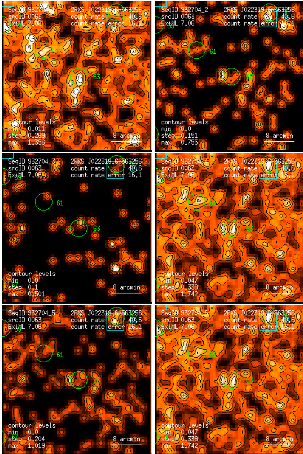
Figure 63: RASS 932704: detection 0063: band rate images, Gaussian filter: (1) PSPC channels 11 – 41, (2) 52 – 90, (3) 91 – 201, (4) 11 – 235, (5) 52 – 201, (6) 11 – 201. Broad band rates in counts/ks. Band rate contour levels in counts/ks/arcmin 2 .
