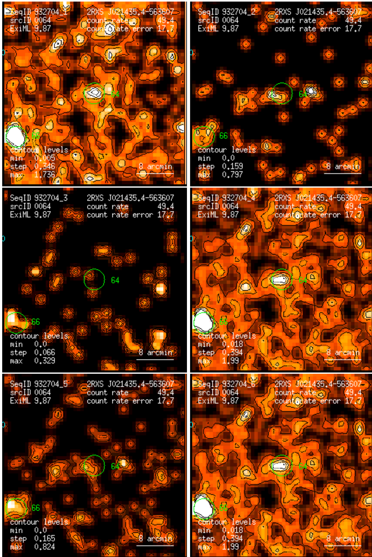
Figure 64: RASS 932704: detection 0064: band rate images, Gaussian filter: (1) PSPC channels 11 – 41, (2) 52 – 90, (3) 91 – 201, (4) 11 – 235, (5) 52 – 201, (6) 11 – 201. Broad band rates in counts/ks. Band rate contour levels in counts/ks/arcmin 2 .
