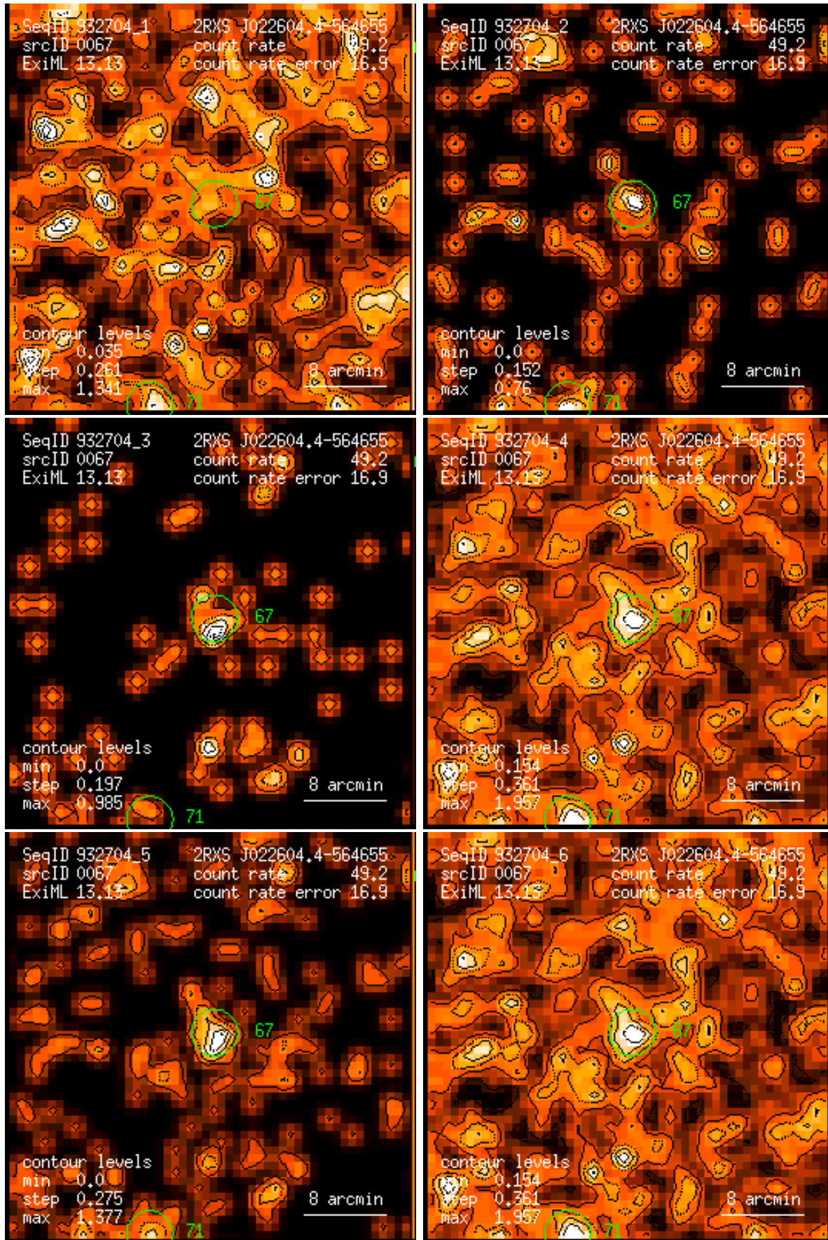
Figure 67: RASS 932704: detection 0067: band rate images, Gaussian filter: (1) PSPC channels 11 – 41, (2) 52 – 90, (3) 91 – 201, (4) 11 – 235, (5) 52 – 201, (6) 11 – 201. Broad band rates in counts/ks. Band rate contour levels in counts/ks/arcmin 2 .
