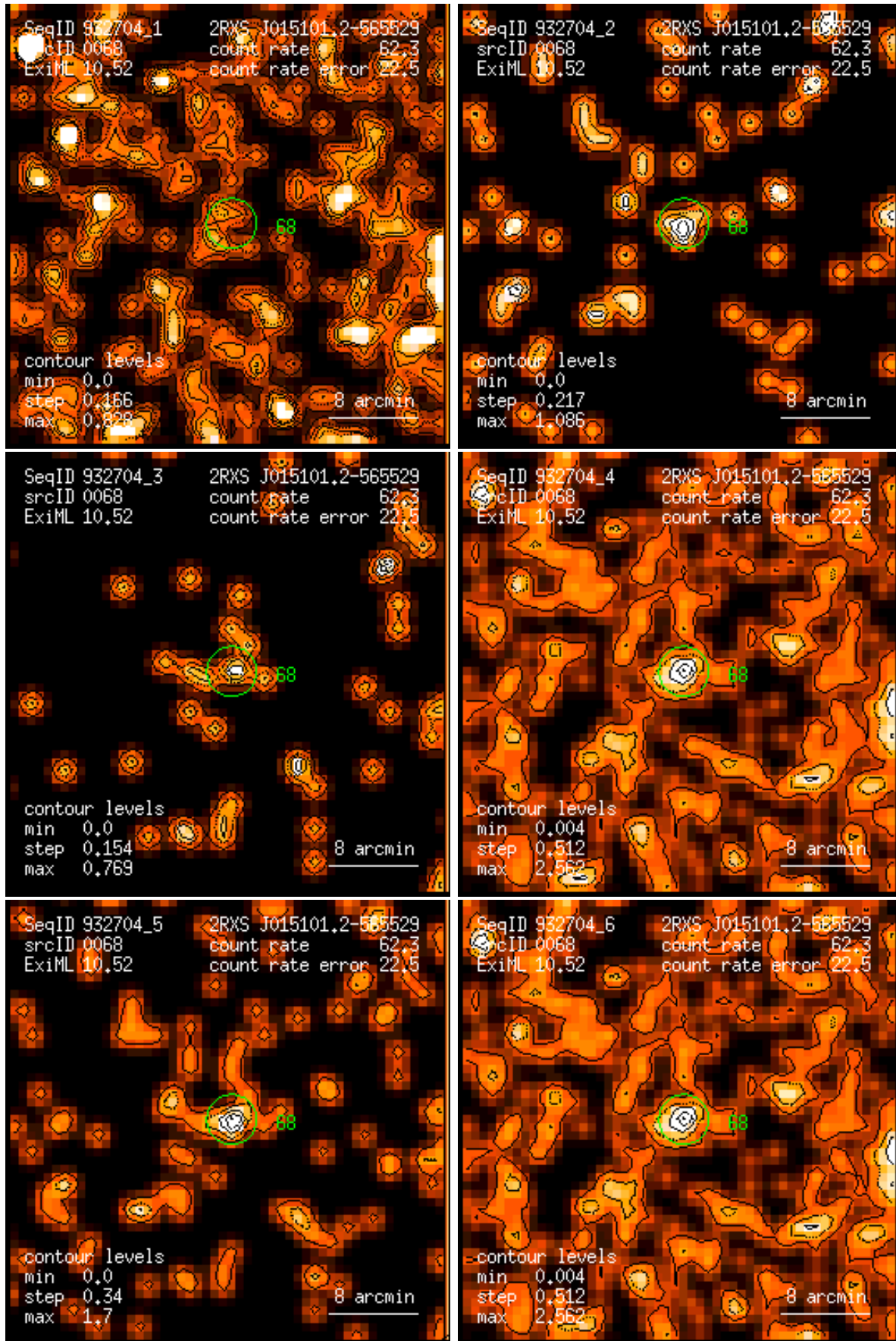
Figure 68: RASS 932704: detection 0068: band rate images, Gaussian filter: (1) PSPC channels 11 – 41, (2) 52 – 90, (3) 91 – 201, (4) 11 – 235, (5) 52 – 201, (6) 11 – 201. Broad band rates in counts/ks. Band rate contour levels in counts/ks/arcmin 2 .
