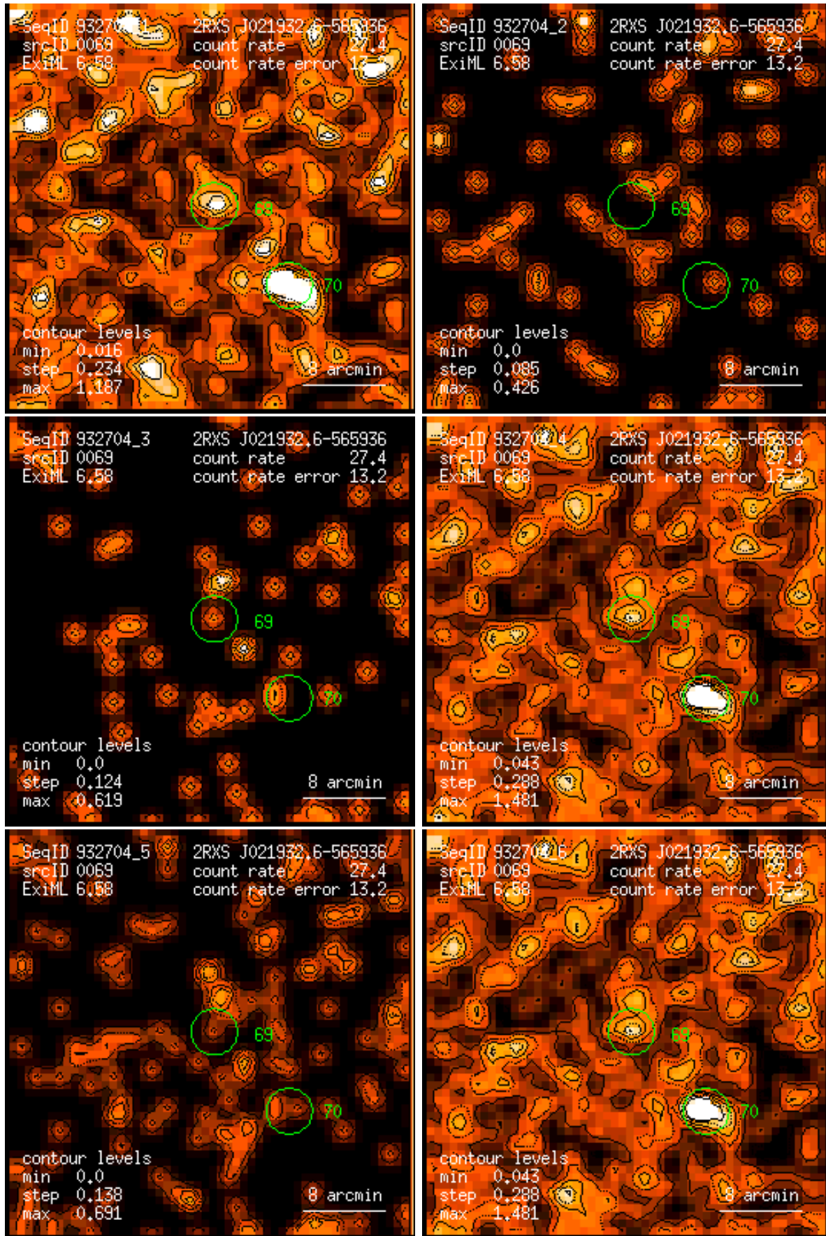
Figure 69: RASS 932704: detection 0069: band rate images, Gaussian filter: (1) PSPC channels 11 – 41, (2) 52 – 90, (3) 91 – 201, (4) 11 – 235, (5) 52 – 201, (6) 11 – 201. Broad band rates in counts/ks. Band rate contour levels in counts/ks/arcmin 2 .
