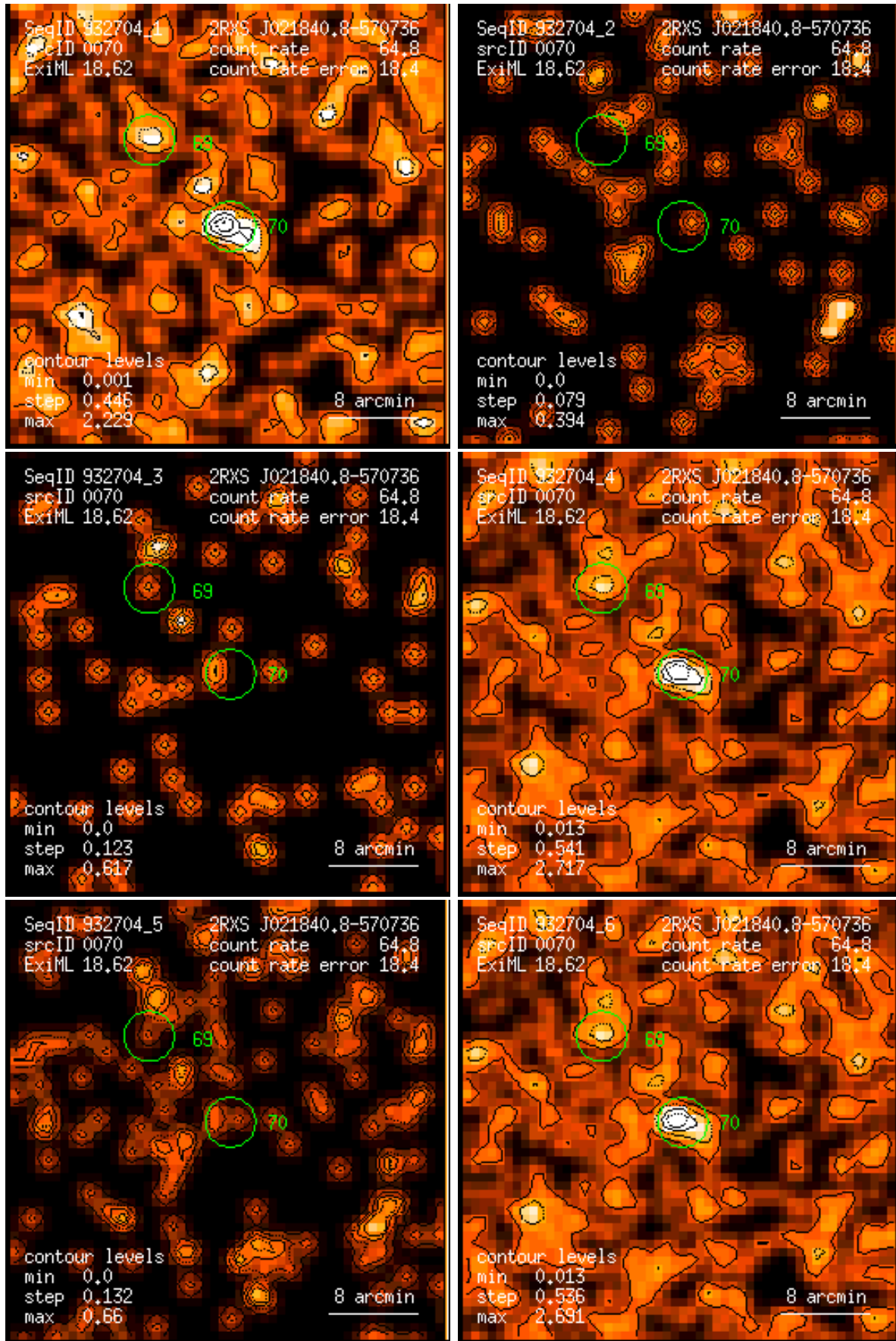
Figure 70: RASS 932704: detection 0070: band rate images, Gaussian filter: (1) PSPC channels 11 – 41, (2) 52 – 90, (3) 91 – 201, (4) 11 – 235, (5) 52 – 201, (6) 11 – 201. Broad band rates in counts/ks. Band rate contour levels in counts/ks/arcmin 2 .
