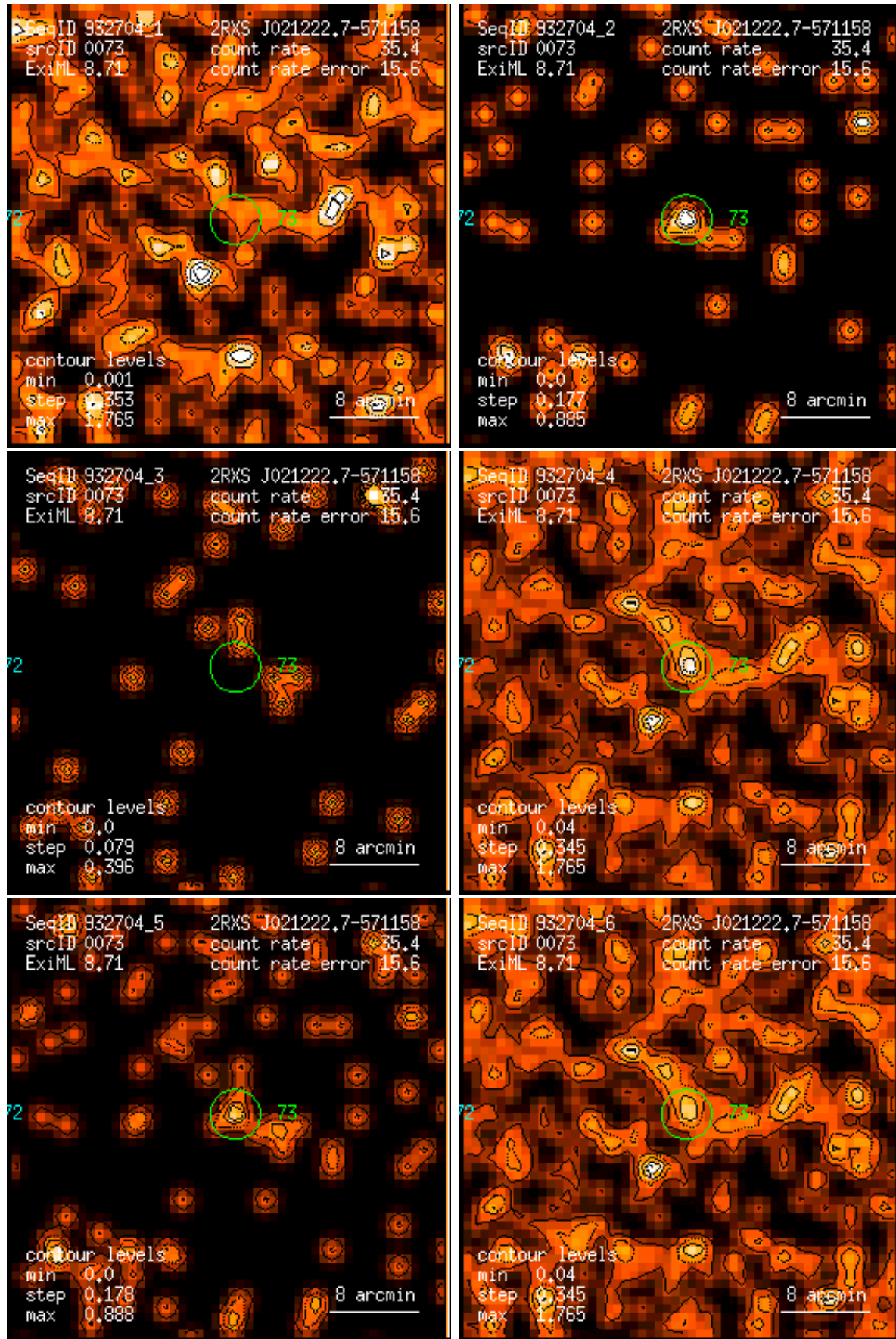
Figure 73: RASS 932704: detection 0073: band rate images, Gaussian filter: (1) PSPC channels 11 – 41, (2) 52 – 90, (3) 91 – 201, (4) 11 – 235, (5) 52 – 201, (6) 11 – 201. Broad band rates in counts/ks. Band rate contour levels in counts/ks/arcmin 2 .
