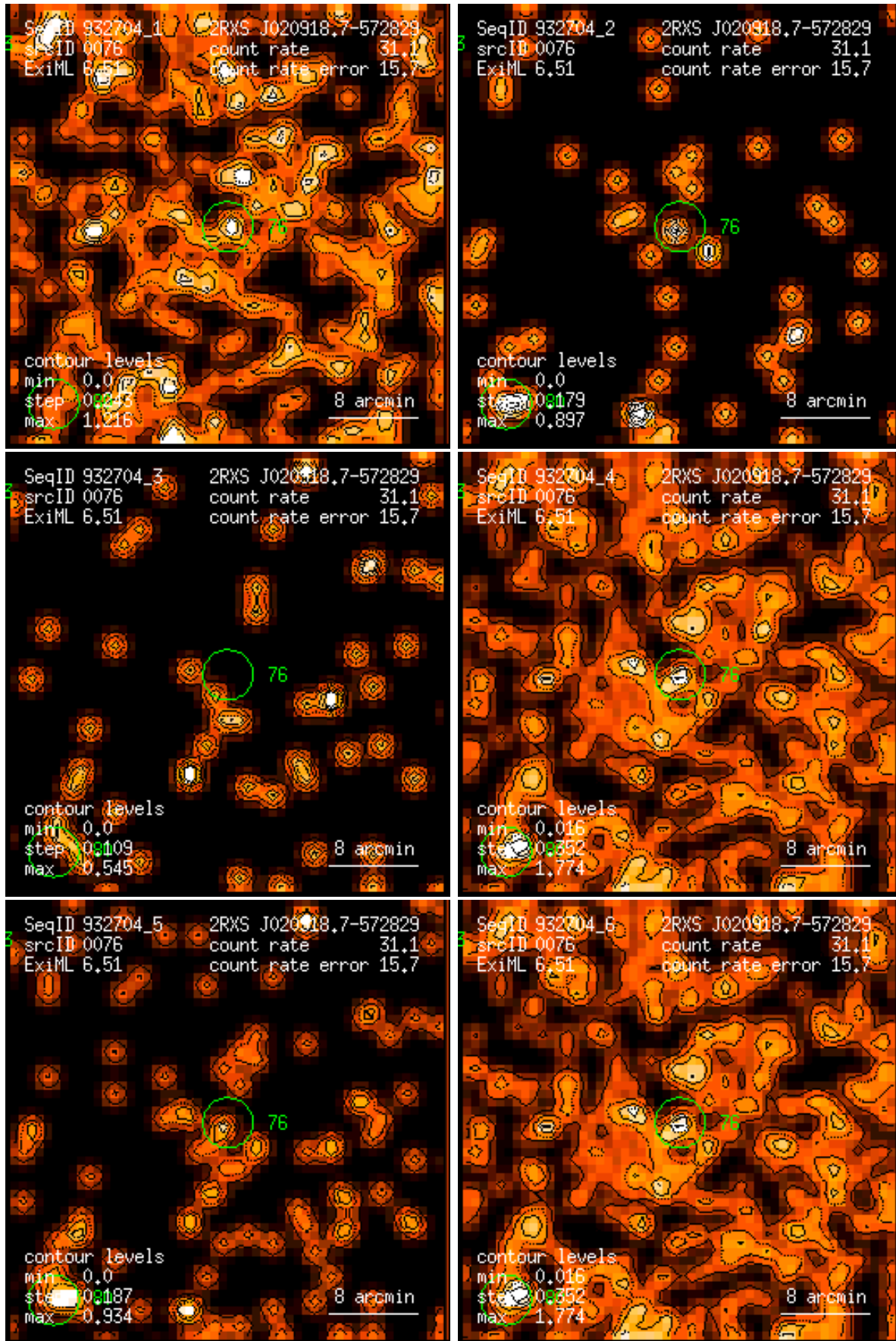
Figure 76: RASS 932704: detection 0076: band rate images, Gaussian filter: (1) PSPC channels 11 – 41, (2) 52 – 90, (3) 91 – 201, (4) 11 – 235, (5) 52 – 201, (6) 11 – 201. Broad band rates in counts/ks. Band rate contour levels in counts/ks/arcmin 2 .
