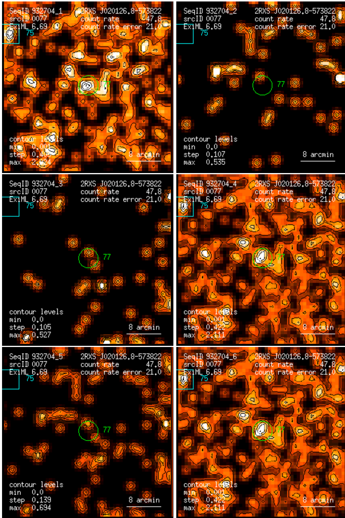
Figure 77: RASS 932704: detection 0077: band rate images, Gaussian filter: (1) PSPC channels 11 – 41, (2) 52 – 90, (3) 91 – 201, (4) 11 – 235, (5) 52 – 201, (6) 11 – 201. Broad band rates in counts/ks. Band rate contour levels in counts/ks/arcmin 2 .
