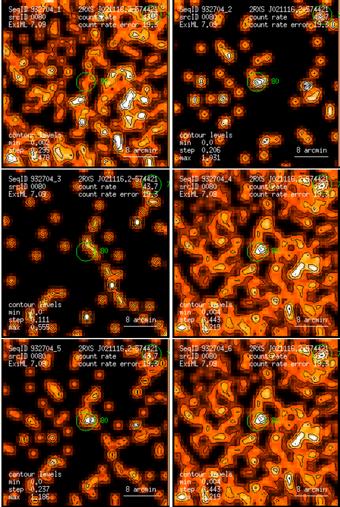
Figure 80: RASS 932704: detection 0080: band rate images, Gaussian filter: (1) PSPC channels 11 – 41, (2) 52 – 90, (3) 91 – 201, (4) 11 – 235, (5) 52 – 201, (6) 11 – 201. Broad band rates in counts/ks. Band rate contour levels in counts/ks/arcmin 2 .
