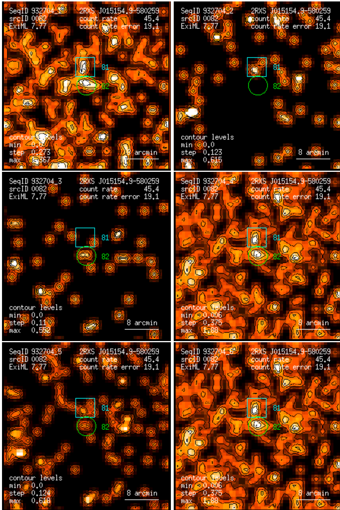
Figure 82: RASS 932704: detection 0082: band rate images, Gaussian filter: (1) PSPC channels 11 – 41, (2) 52 – 90, (3) 91 – 201, (4) 11 – 235, (5) 52 – 201, (6) 11 – 201. Broad band rates in counts/ks. Band rate contour levels in counts/ks/arcmin 2 .
