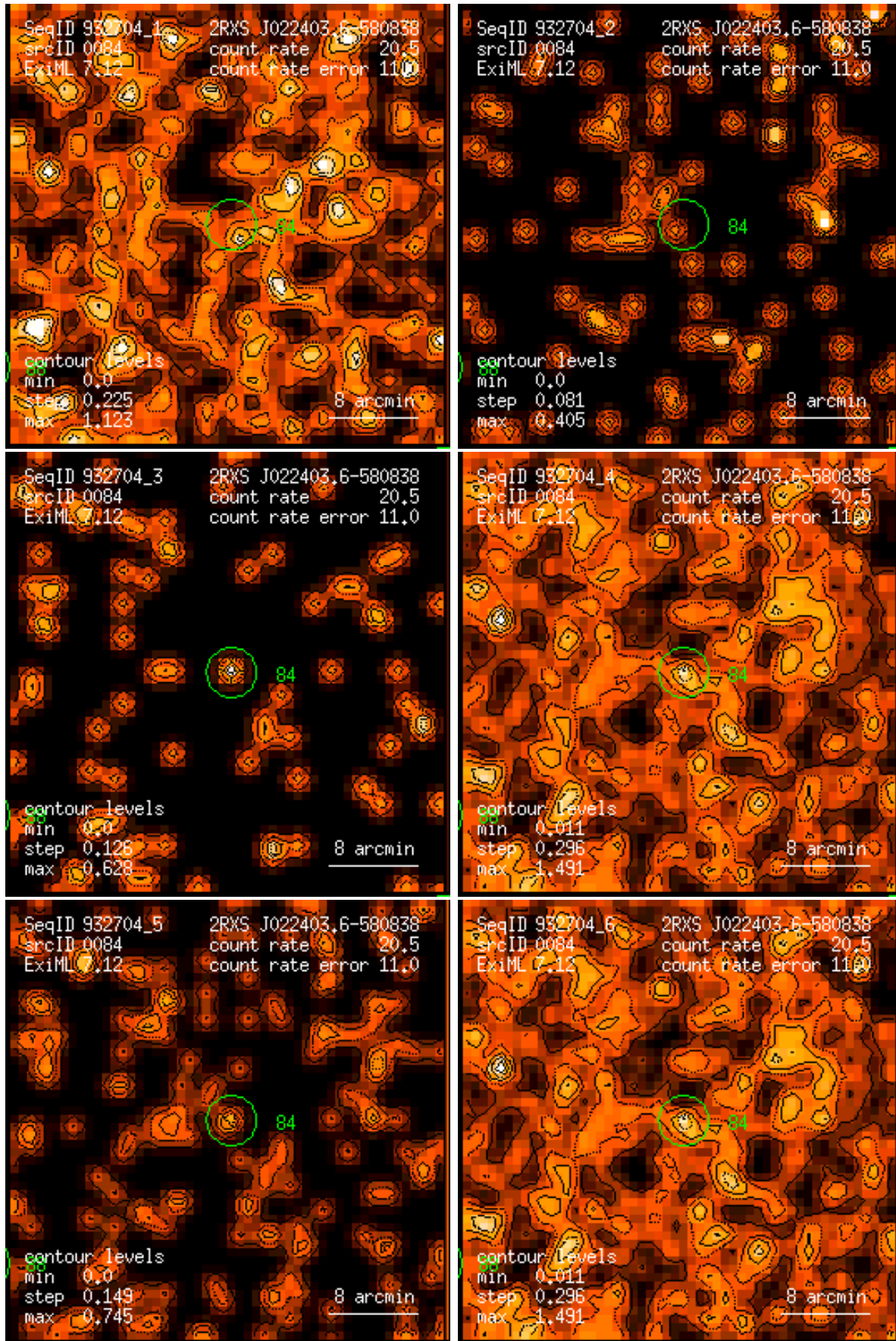
Figure 84: RASS 932704: detection 0084: band rate images, Gaussian filter: (1) PSPC channels 11 – 41, (2) 52 – 90, (3) 91 – 201, (4) 11 – 235, (5) 52 – 201, (6) 11 – 201. Broad band rates in counts/ks. Band rate contour levels in counts/ks/arcmin 2 .
