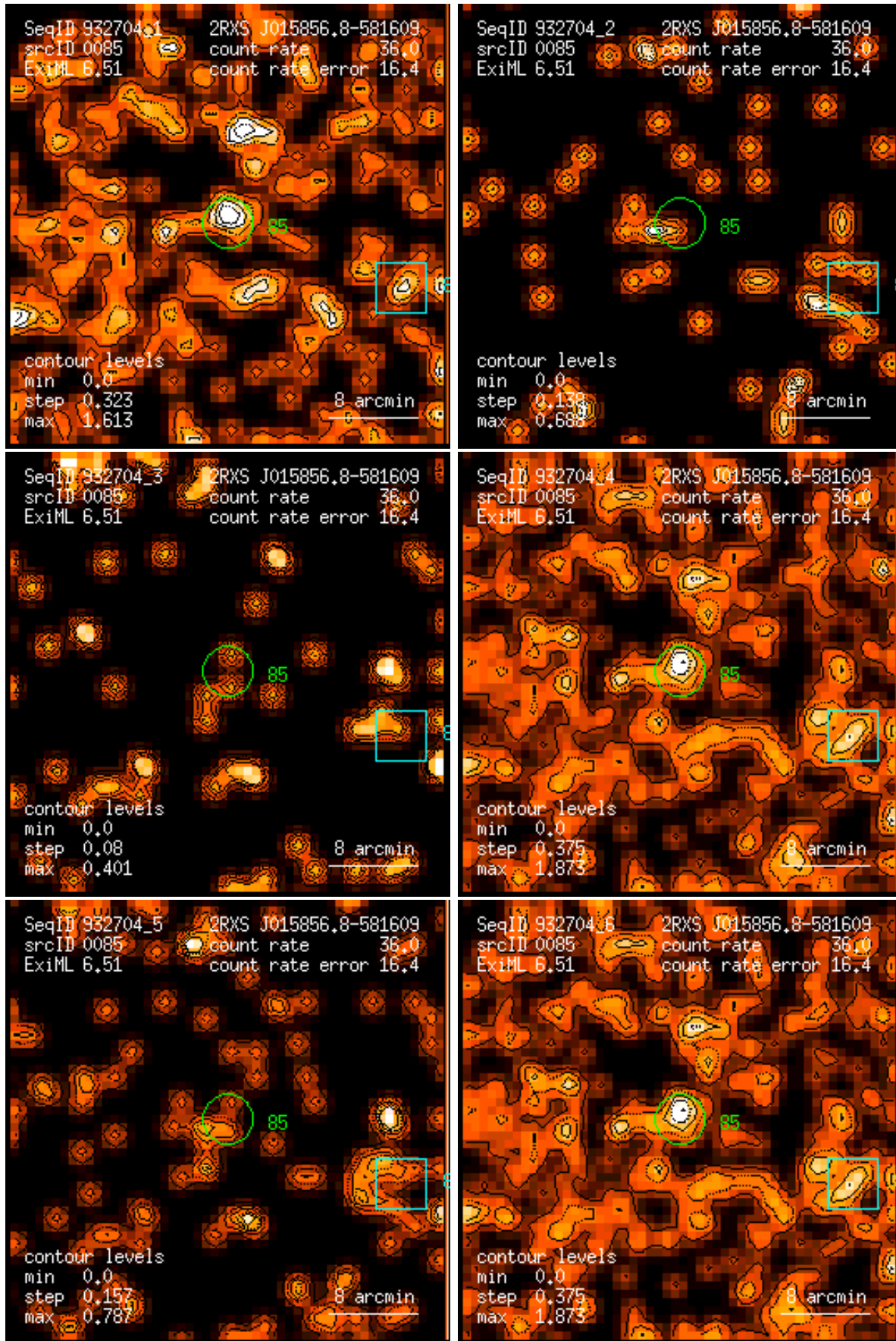
Figure 85: RASS 932704: detection 0085: band rate images, Gaussian filter: (1) PSPC channels 11 – 41, (2) 52 – 90, (3) 91 – 201, (4) 11 – 235, (5) 52 – 201, (6) 11 – 201. Broad band rates in counts/ks. Band rate contour levels in counts/ks/arcmin 2 .
