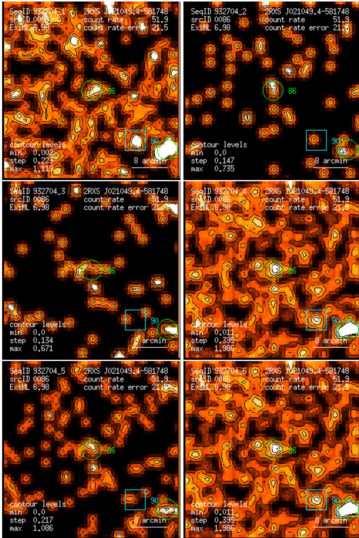
Figure 86: RASS 932704: detection 0086: band rate images, Gaussian filter: (1) PSPC channels 11 – 41, (2) 52 – 90, (3) 91 – 201, (4) 11 – 235, (5) 52 – 201, (6) 11 – 201. Broad band rates in counts/ks. Band rate contour levels in counts/ks/arcmin 2 .
