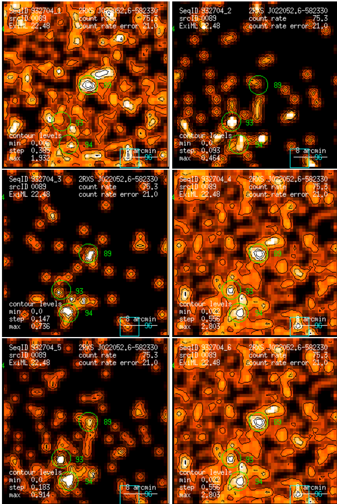
Figure 89: RASS 932704: detection 0089: band rate images, Gaussian filter: (1) PSPC channels 11 – 41, (2) 52 – 90, (3) 91 – 201, (4) 11 – 235, (5) 52 – 201, (6) 11 – 201. Broad band rates in counts/ks. Band rate contour levels in counts/ks/arcmin 2 .
