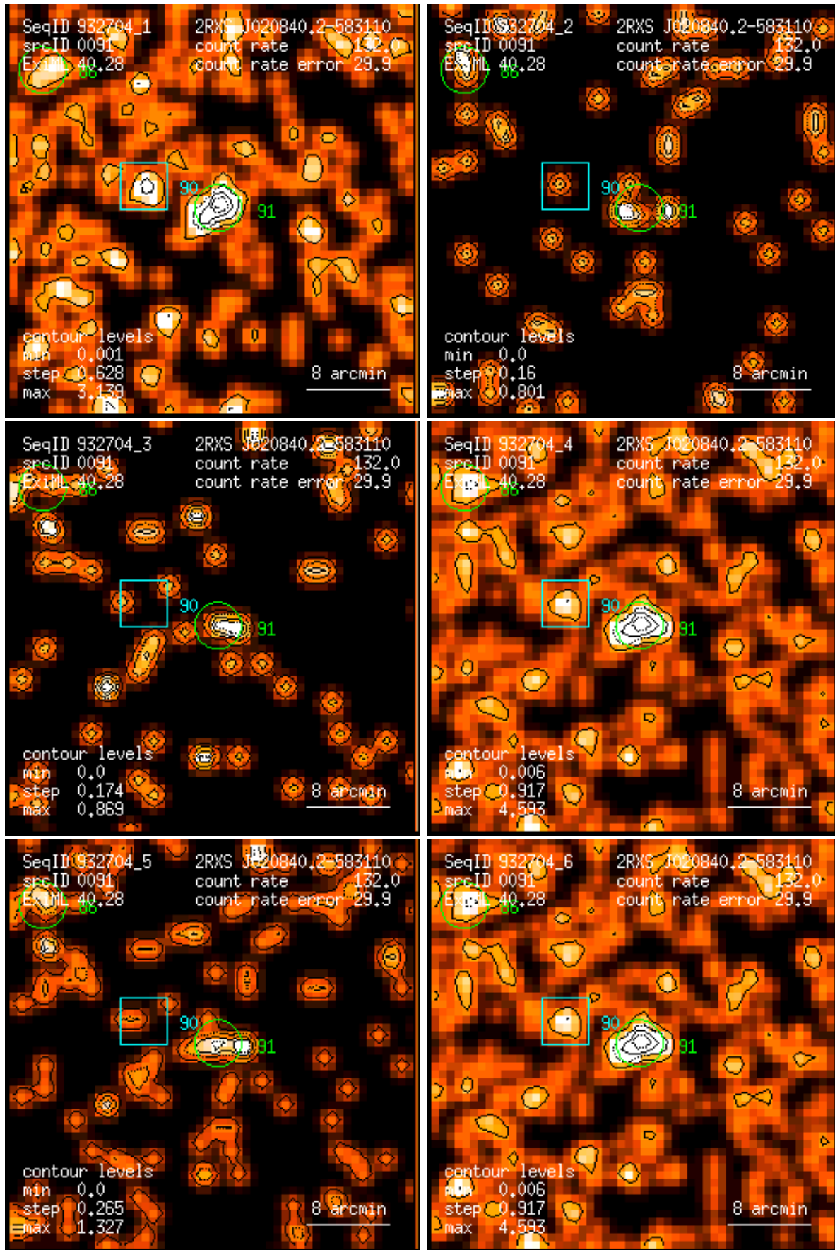
Figure 91: RASS 932704: detection 0091: band rate images, Gaussian filter: (1) PSPC channels 11 – 41, (2) 52 – 90, (3) 91 – 201, (4) 11 – 235, (5) 52 – 201, (6) 11 – 201. Broad band rates in counts/ks. Band rate contour levels in counts/ks/arcmin 2 .
