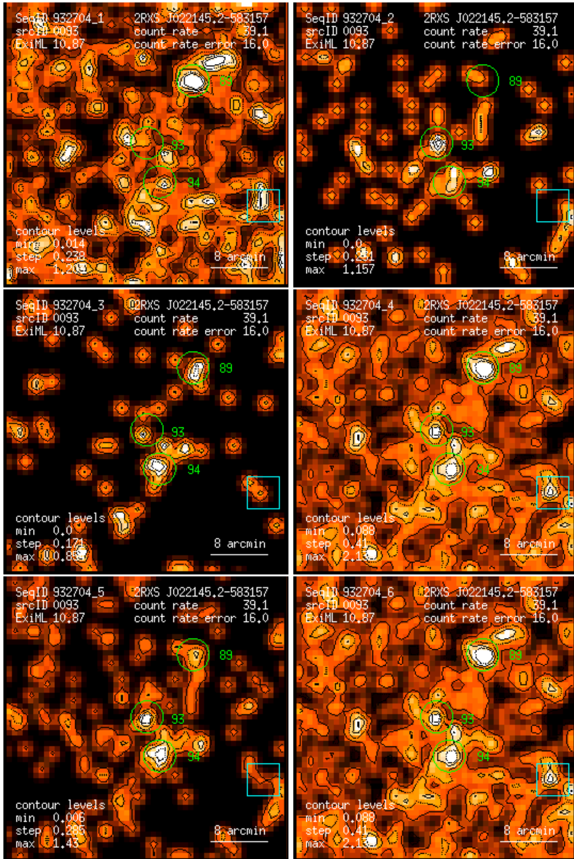
Figure 93: RASS 932704: detection 0093: band rate images, Gaussian filter: (1) PSPC channels 11 – 41, (2) 52 – 90, (3) 91 – 201, (4) 11 – 235, (5) 52 – 201, (6) 11 – 201. Broad band rates in counts/ks. Band rate contour levels in counts/ks/arcmin 2 .
