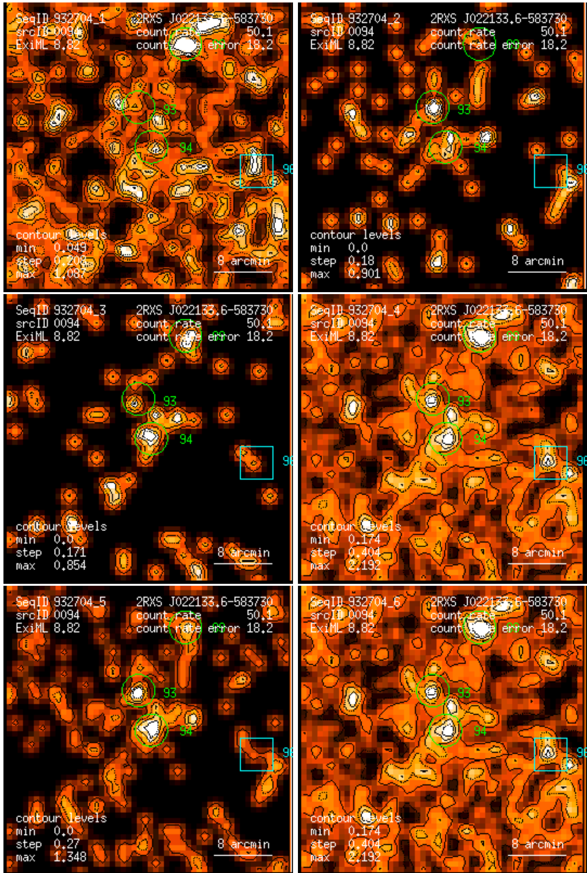
Figure 94: RASS 932704: detection 0094: band rate images, Gaussian filter: (1) PSPC channels 11 – 41, (2) 52 – 90, (3) 91 – 201, (4) 11 – 235, (5) 52 – 201, (6) 11 – 201. Broad band rates in counts/ks. Band rate contour levels in counts/ks/arcmin 2 .
