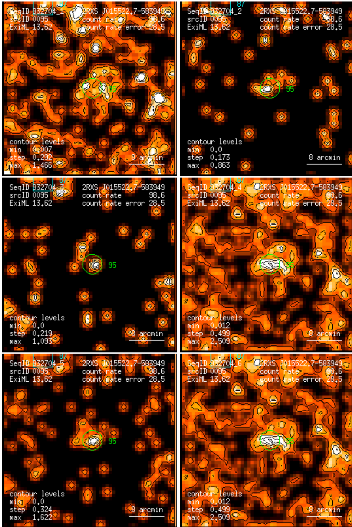
Figure 95: RASS 932704: detection 0095: band rate images, Gaussian filter: (1) PSPC channels 11 – 41, (2) 52 – 90, (3) 91 – 201, (4) 11 – 235, (5) 52 – 201, (6) 11 – 201. Broad band rates in counts/ks. Band rate contour levels in counts/ks/arcmin 2 .
