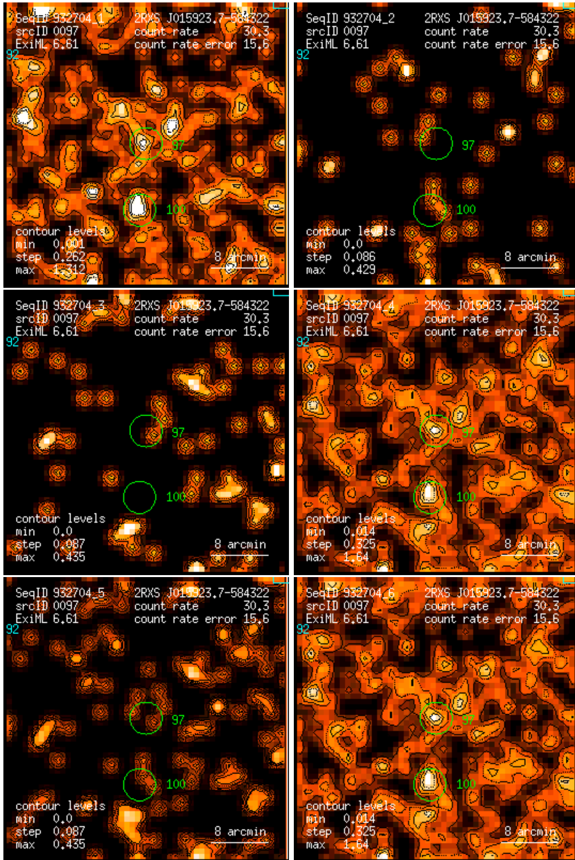
Figure 97: RASS 932704: detection 0097: band rate images, Gaussian filter: (1) PSPC channels 11 – 41, (2) 52 – 90, (3) 91 – 201, (4) 11 – 235, (5) 52 – 201, (6) 11 – 201. Broad band rates in counts/ks. Band rate contour levels in counts/ks/arcmin 2 .
