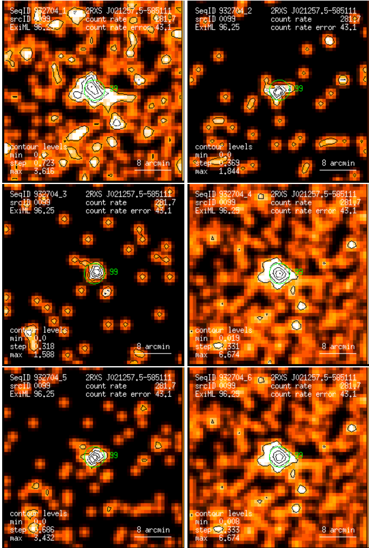
Figure 99: RASS 932704: detection 0099: band rate images, Gaussian filter: (1) PSPC channels 11 – 41, (2) 52 – 90, (3) 91 – 201, (4) 11 – 235, (5) 52 – 201, (6) 11 – 201. Broad band rates in counts/ks. Band rate contour levels in counts/ks/arcmin 2 .
