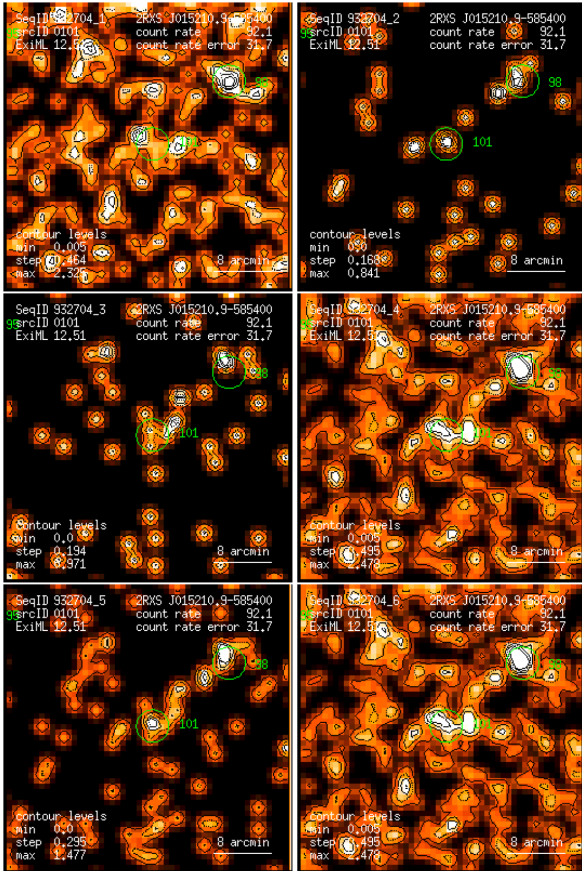
Figure 101: RASS 932704: detection 0101: band rate images, Gaussian filter: (1) PSPC channels 11 – 41, (2) 52 – 90, (3) 91 – 201, (4) 11 – 235, (5) 52 – 201, (6) 11 – 201. Broad band rates in counts/ks. Band rate contour levels in counts/ks/arcmin 2 .
