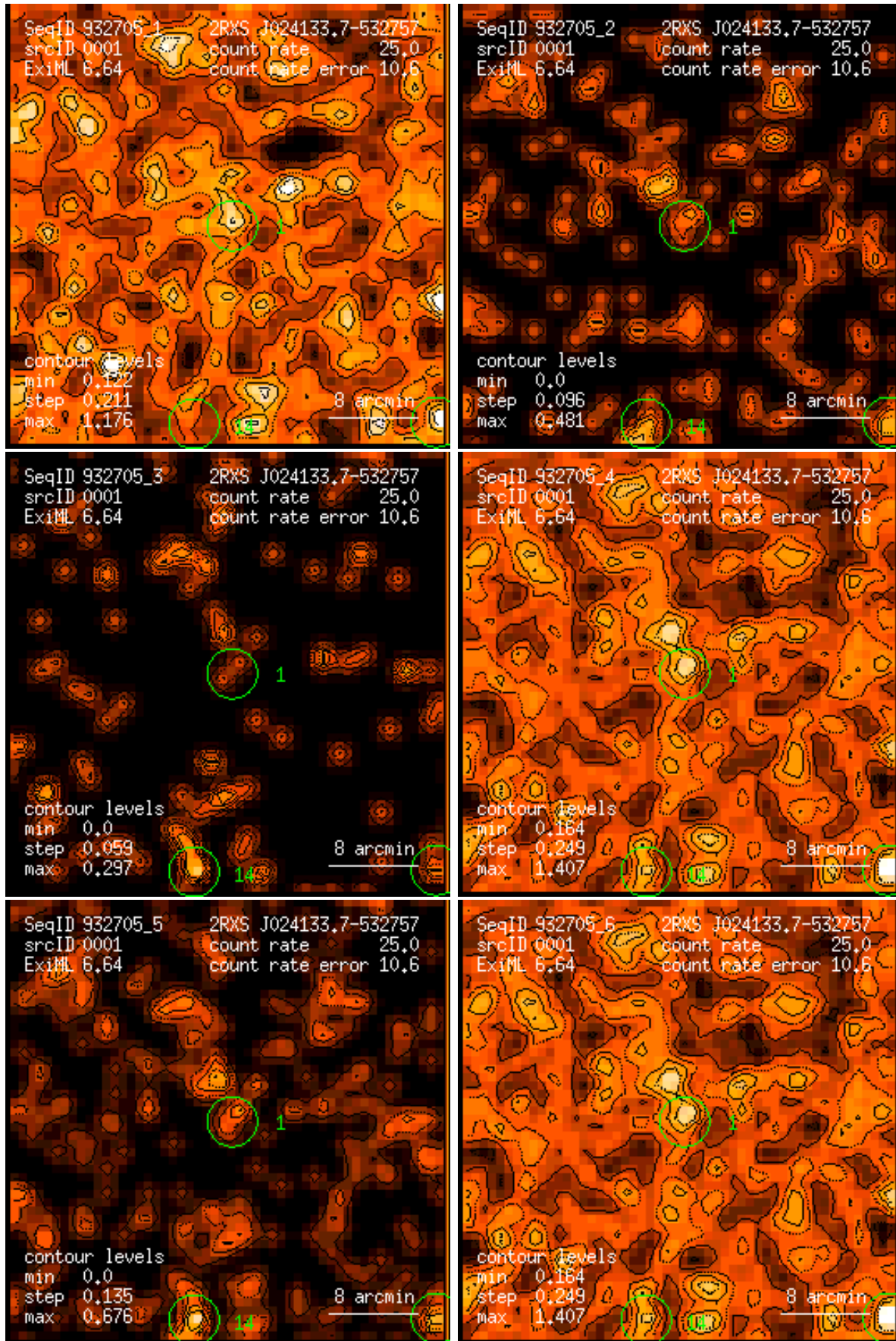
Figure 1: RASS 932705: detection 0001: band rate images, Gaussian filter: (1) PSPC channels 11 – 41, (2) 52 – 90, (3) 91 – 201, (4) 11 – 235, (5) 52 – 201, (6) 11 – 201. Broad band rates in counts/ks. Band rate contour levels in counts/ks/arcmin 2 .
