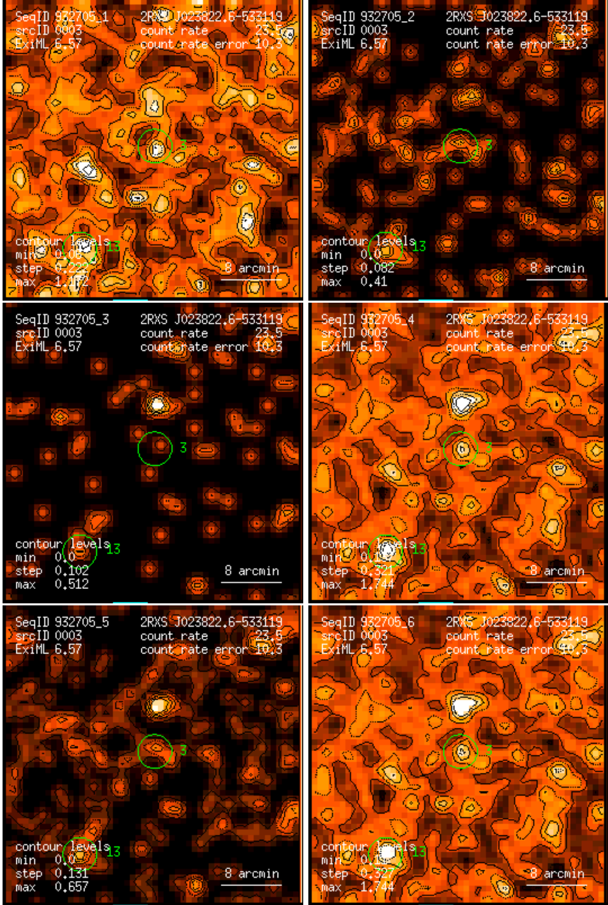
Figure 3: RASS 932705: detection 0003: band rate images, Gaussian filter: (1) PSPC channels 11 – 41, (2) 52 – 90, (3) 91 – 201, (4) 11 – 235, (5) 52 – 201, (6) 11 – 201. Broad band rates in counts/ks. Band rate contour levels in counts/ks/arcmin 2 .
