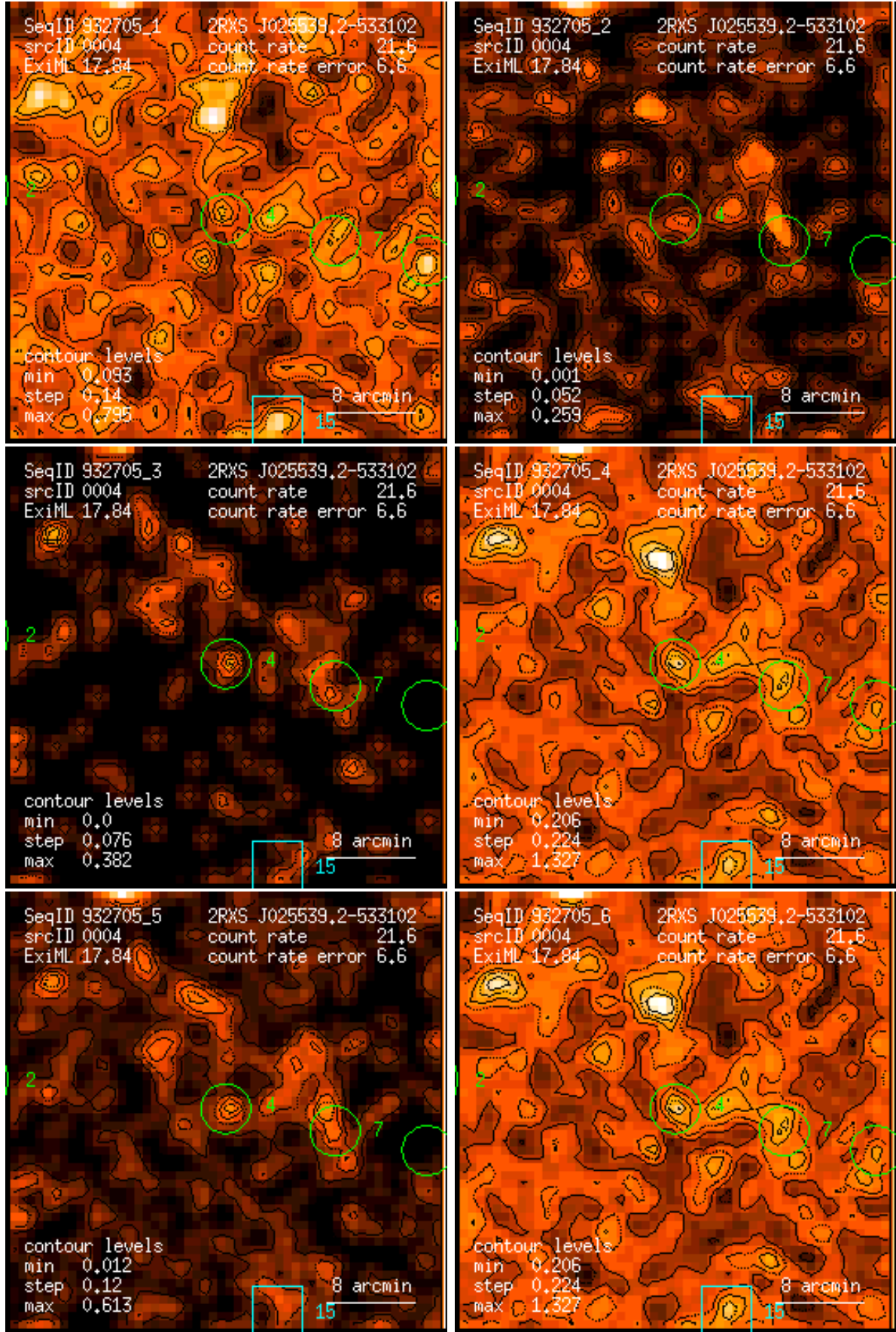
Figure 4: RASS 932705: detection 0004: band rate images, Gaussian filter: (1) PSPC channels 11 – 41, (2) 52 – 90, (3) 91 – 201, (4) 11 – 235, (5) 52 – 201, (6) 11 – 201. Broad band rates in counts/ks. Band rate contour levels in counts/ks/arcmin 2 .
