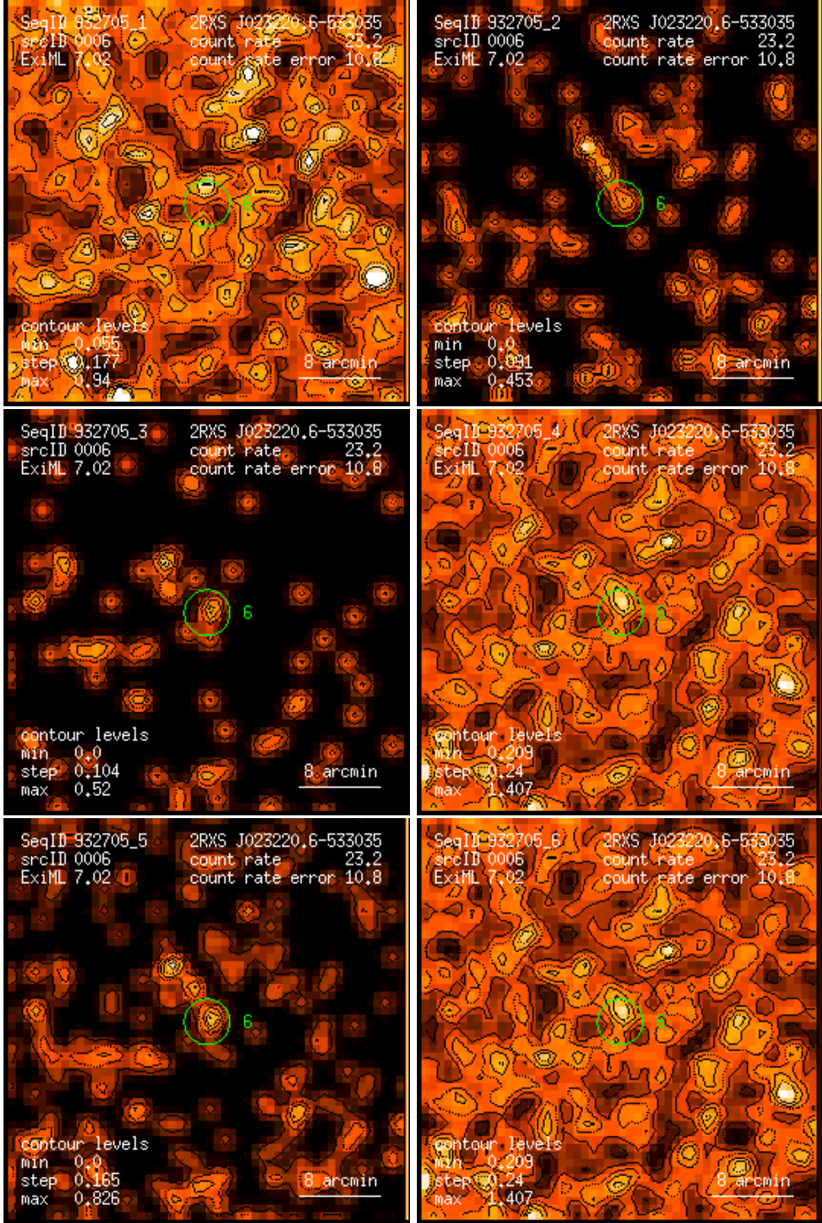
Figure 6: RASS 932705: detection 0006: band rate images, Gaussian filter: (1) PSPC channels 11 – 41, (2) 52 – 90, (3) 91 – 201, (4) 11 – 235, (5) 52 – 201, (6) 11 – 201. Broad band rates in counts/ks. Band rate contour levels in counts/ks/arcmin 2 .
