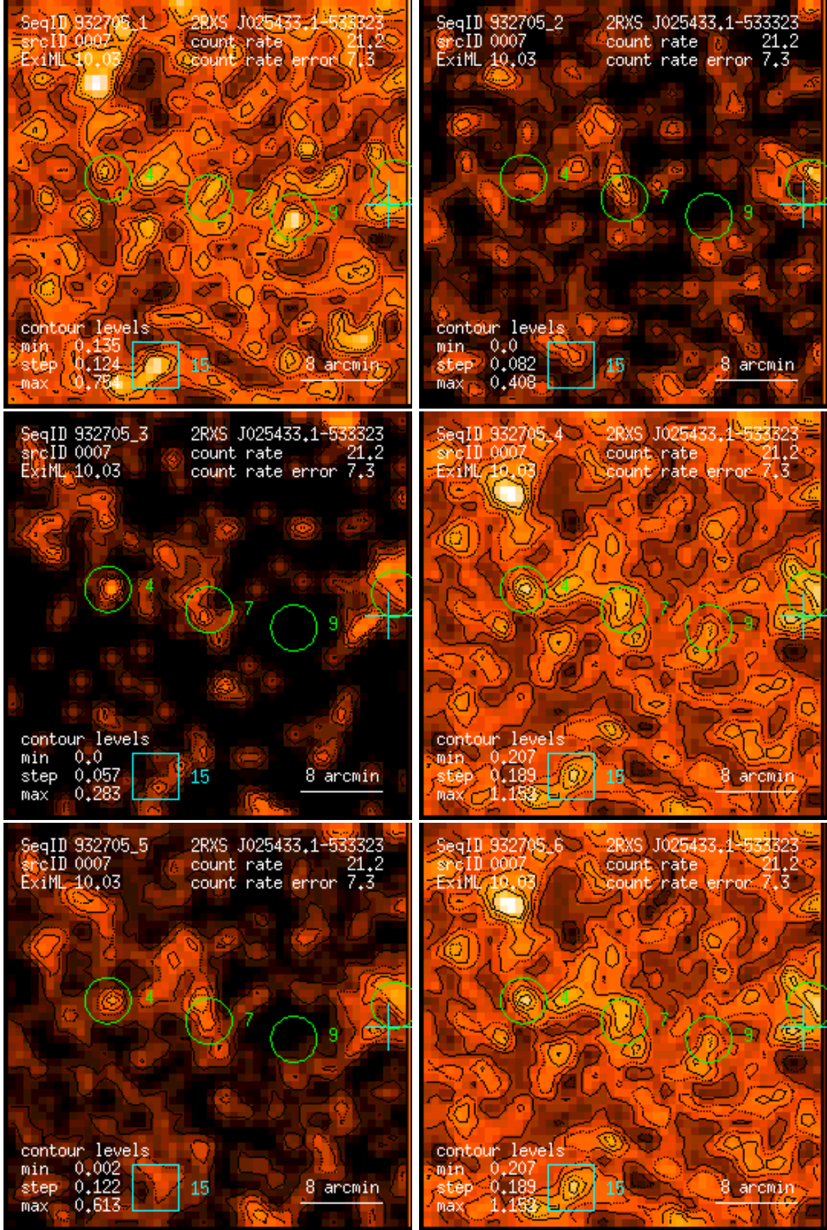
Figure 7: RASS 932705: detection 0007: band rate images, Gaussian filter: (1) PSPC channels 11 – 41, (2) 52 – 90, (3) 91 – 201, (4) 11 – 235, (5) 52 – 201, (6) 11 – 201. Broad band rates in counts/ks. Band rate contour levels in counts/ks/arcmin 2 .
