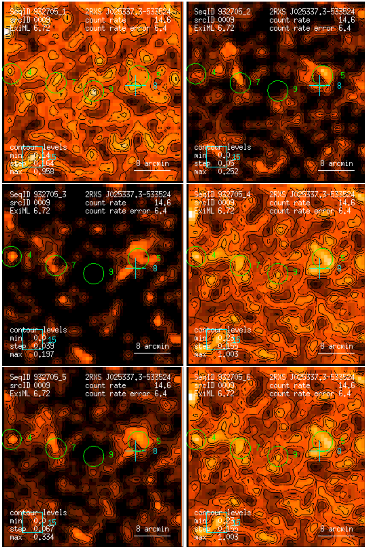
Figure 9: RASS 932705: detection 0009: band rate images, Gaussian filter: (1) PSPC channels 11 – 41, (2) 52 – 90, (3) 91 – 201, (4) 11 – 235, (5) 52 – 201, (6) 11 – 201. Broad band rates in counts/ks. Band rate contour levels in counts/ks/arcmin 2 .
