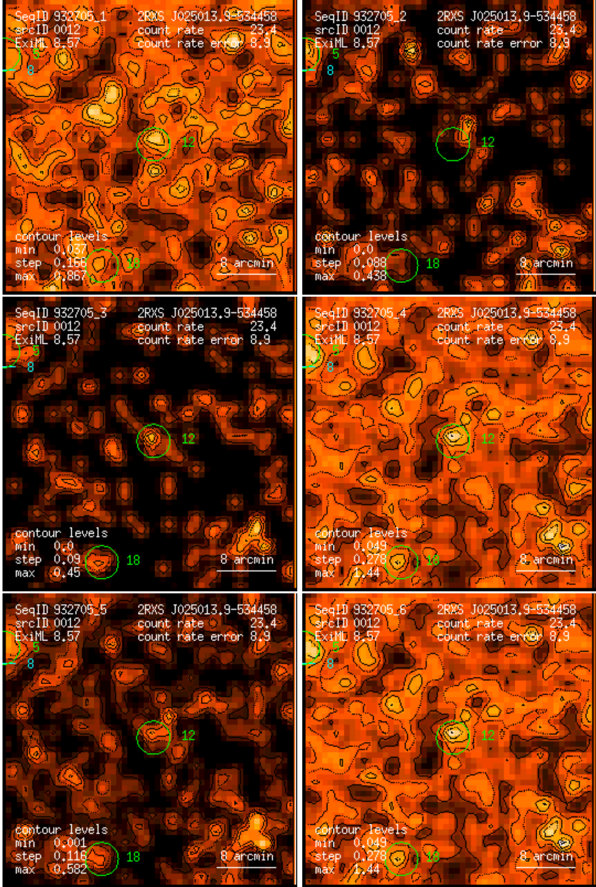
Figure 12: RASS 932705: detection 0012: band rate images, Gaussian filter: (1) PSPC channels 11 – 41, (2) 52 – 90, (3) 91 – 201, (4) 11 – 235, (5) 52 – 201, (6) 11 – 201. Broad band rates in counts/ks. Band rate contour levels in counts/ks/arcmin 2 .
