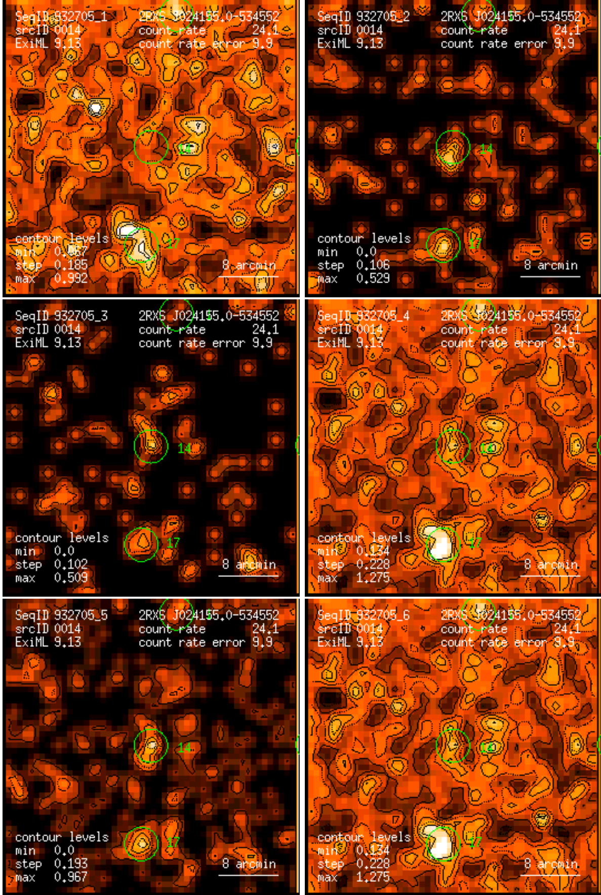
Figure 14: RASS 932705: detection 0014: band rate images, Gaussian filter: (1) PSPC channels 11 – 41, (2) 52 – 90, (3) 91 – 201, (4) 11 – 235, (5) 52 – 201, (6) 11 – 201. Broad band rates in counts/ks. Band rate contour levels in counts/ks/arcmin 2 .
