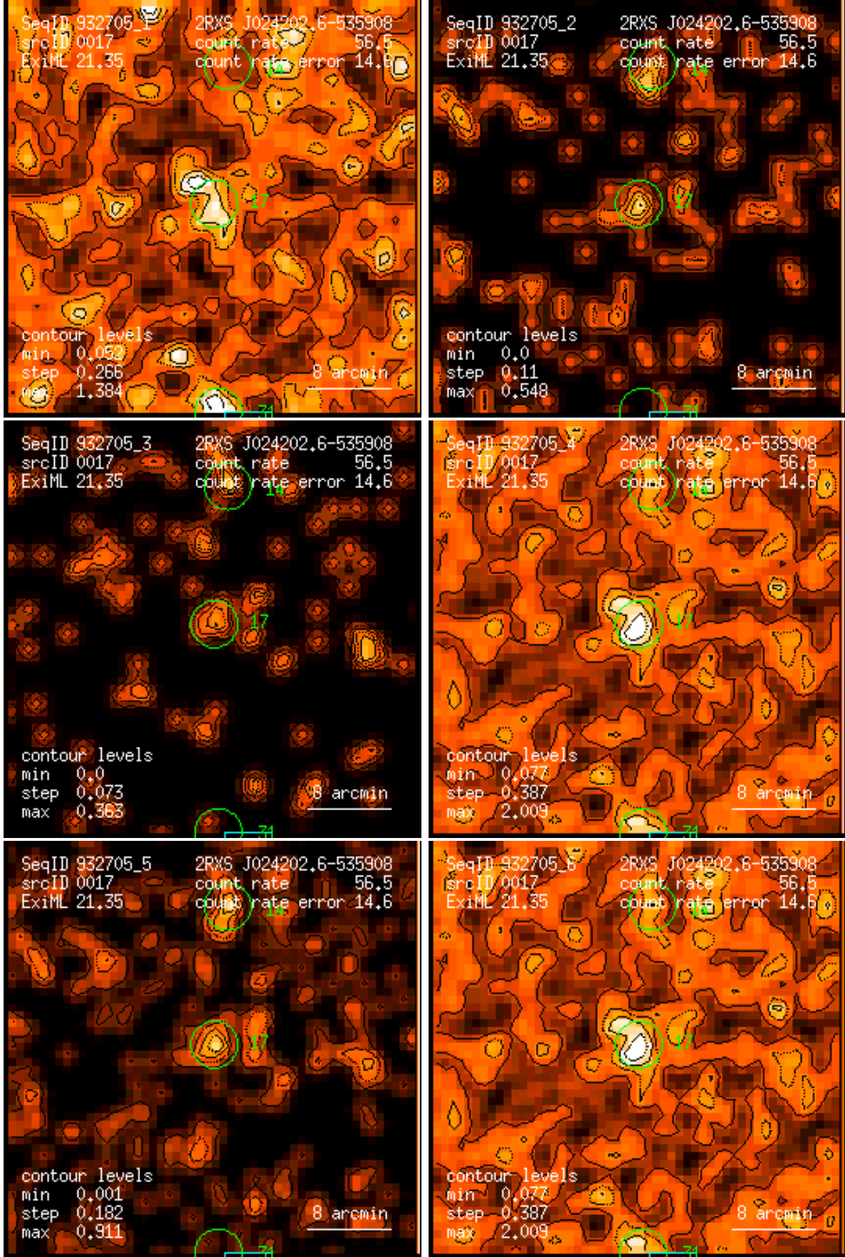
Figure 17: RASS 932705: detection 0017: band rate images, Gaussian filter: (1) PSPC channels 11 – 41, (2) 52 – 90, (3) 91 – 201, (4) 11 – 235, (5) 52 – 201, (6) 11 – 201. Broad band rates in counts/ks. Band rate contour levels in counts/ks/arcmin 2 .
