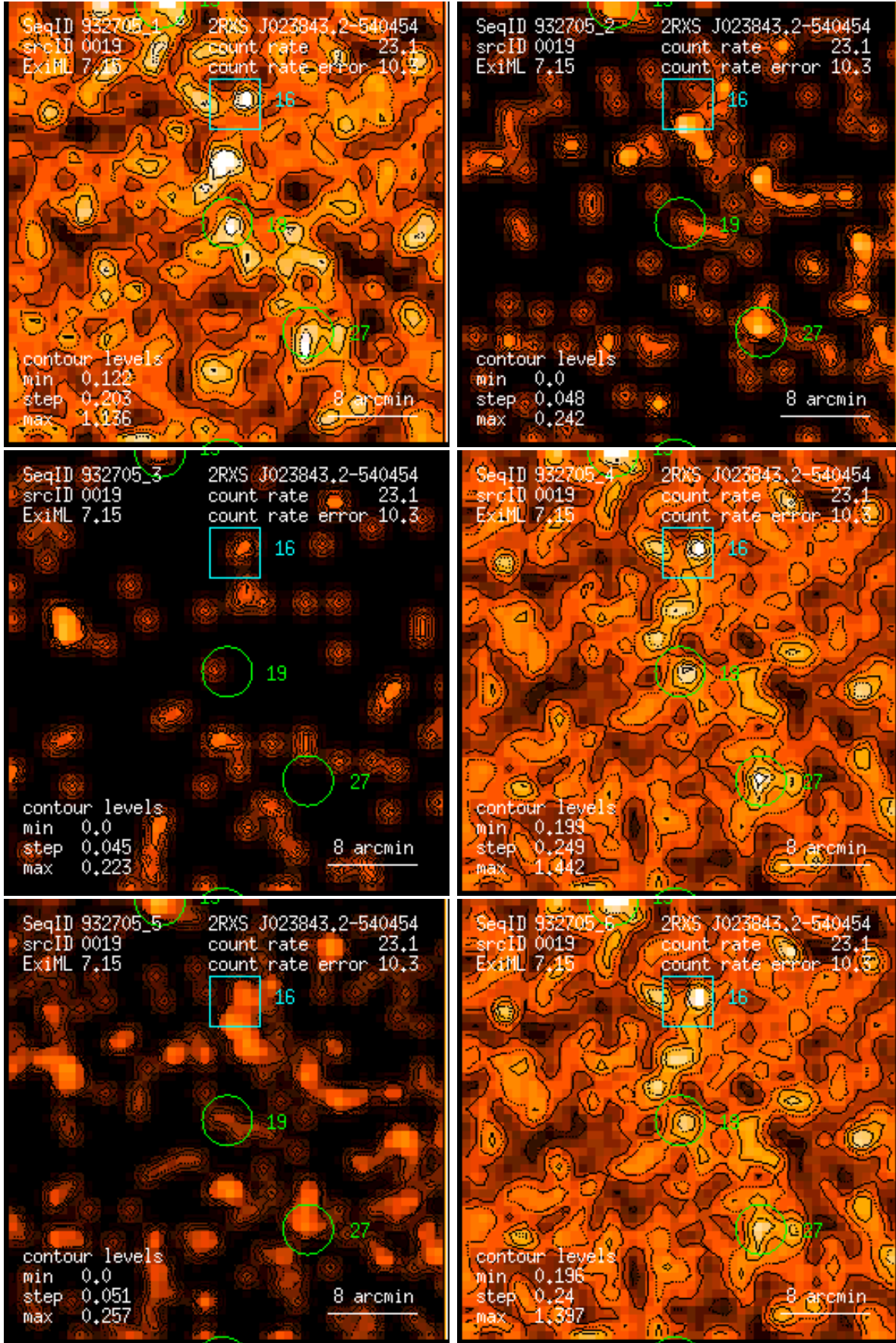
Figure 19: RASS 932705: detection 0019: band rate images, Gaussian filter: (1) PSPC channels 11 – 41, (2) 52 – 90, (3) 91 – 201, (4) 11 – 235, (5) 52 – 201, (6) 11 – 201. Broad band rates in counts/ks. Band rate contour levels in counts/ks/arcmin 2 .
