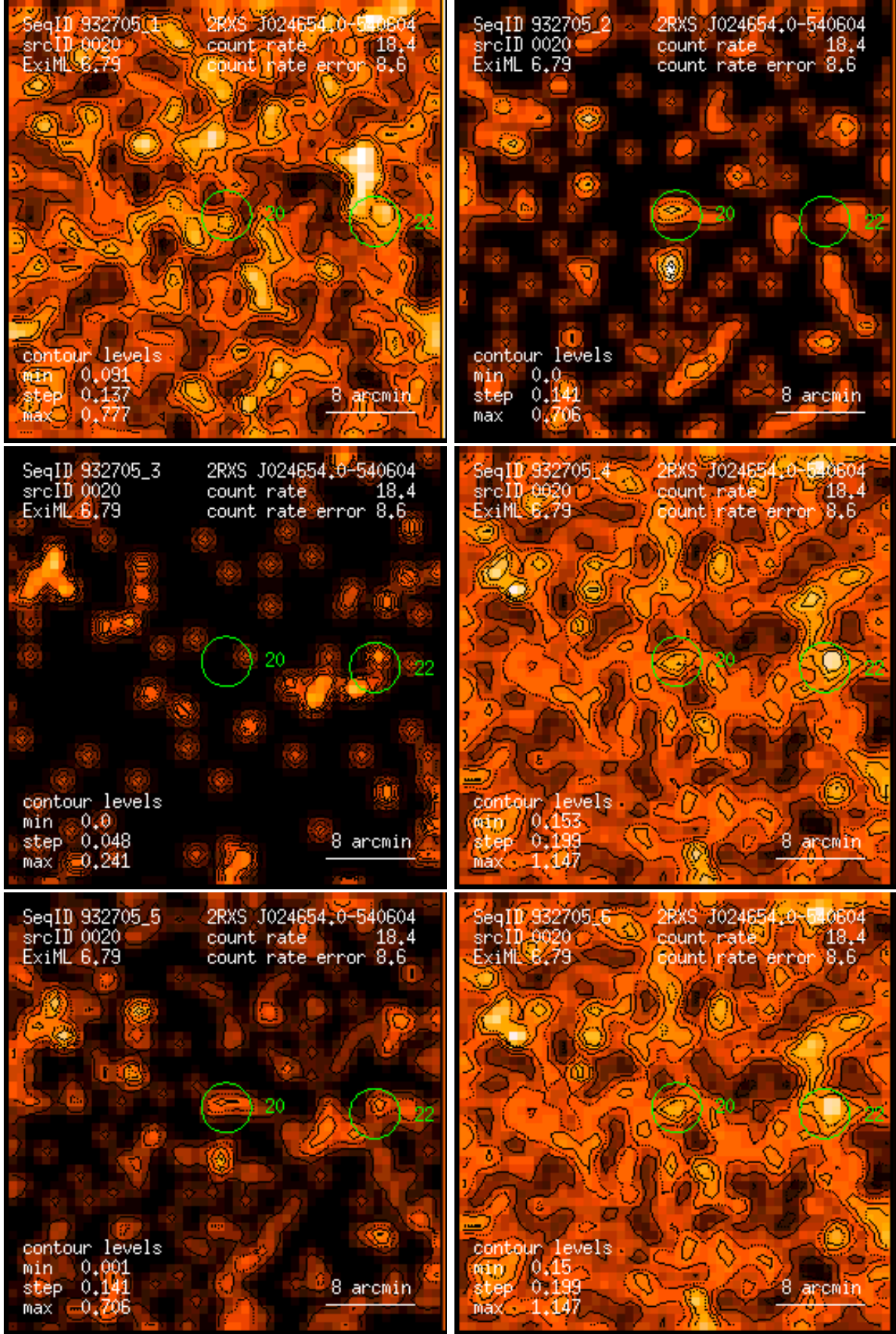
Figure 20: RASS 932705: detection 0020: band rate images, Gaussian filter: (1) PSPC channels 11 – 41, (2) 52 – 90, (3) 91 – 201, (4) 11 – 235, (5) 52 – 201, (6) 11 – 201. Broad band rates in counts/ks. Band rate contour levels in counts/ks/arcmin 2 .
