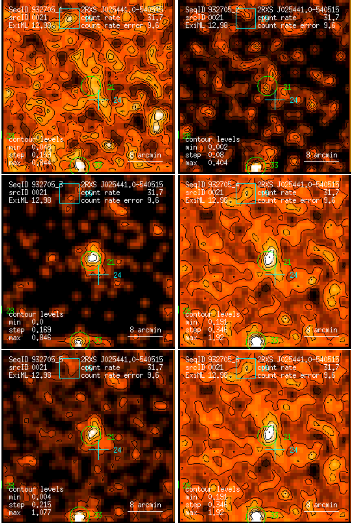
Figure 21: RASS 932705: detection 0021: band rate images, Gaussian filter: (1) PSPC channels 11 – 41, (2) 52 – 90, (3) 91 – 201, (4) 11 – 235, (5) 52 – 201, (6) 11 – 201. Broad band rates in counts/ks. Band rate contour levels in counts/ks/arcmin 2 .
