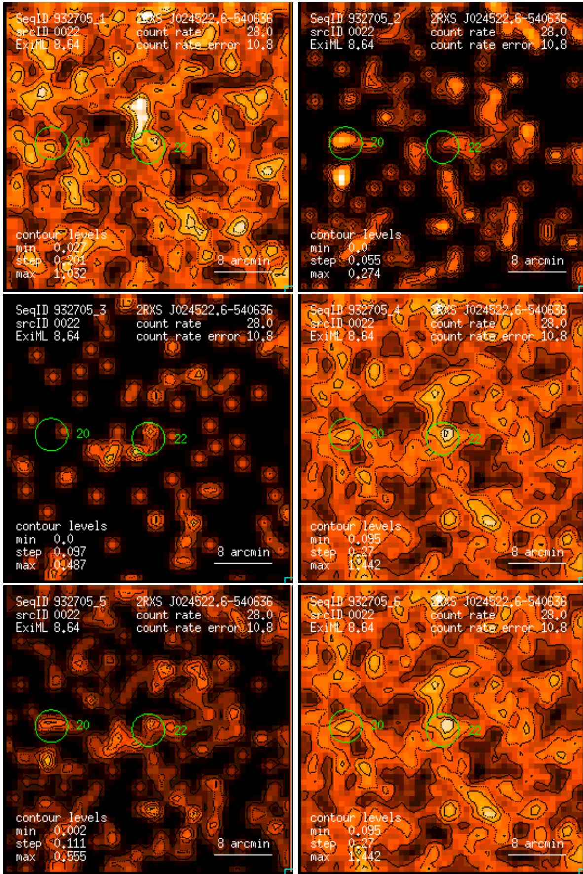
Figure 22: RASS 932705: detection 0022: band rate images, Gaussian filter: (1) PSPC channels 11 – 41, (2) 52 – 90, (3) 91 – 201, (4) 11 – 235, (5) 52 – 201, (6) 11 – 201. Broad band rates in counts/ks. Band rate contour levels in counts/ks/arcmin 2 .
