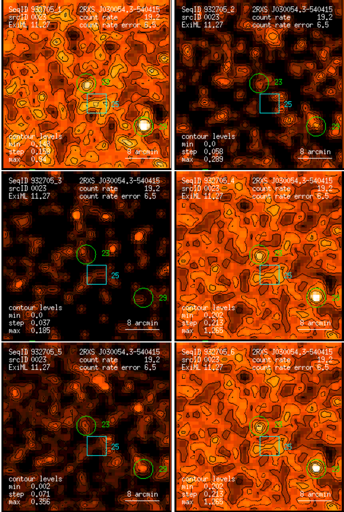
Figure 23: RASS 932705: detection 0023: band rate images, Gaussian filter: (1) PSPC channels 11 – 41, (2) 52 – 90, (3) 91 – 201, (4) 11 – 235, (5) 52 – 201, (6) 11 – 201. Broad band rates in counts/ks. Band rate contour levels in counts/ks/arcmin 2 .
